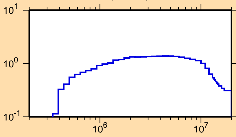
\sigma vs. E for ^{59}\text{Ni}(n,\text{inel.})
