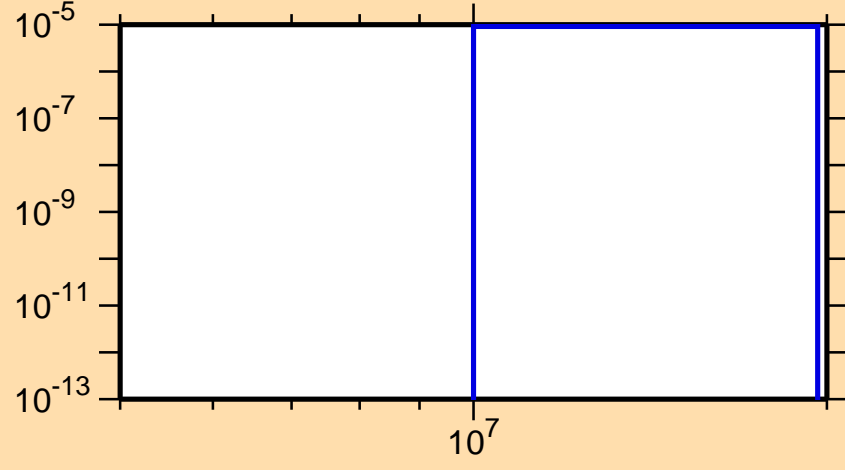
\sigma vs. E for ^{59}\text{Ni}(n,\text{He3})
