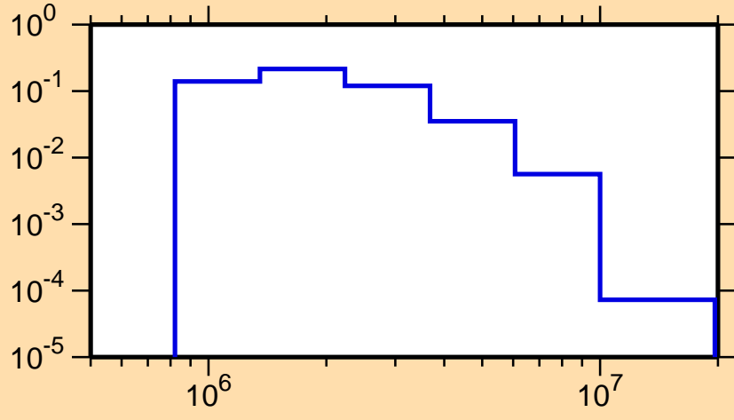
\sigma vs. E for ^{59}\text{Ni}(n,n_3)
