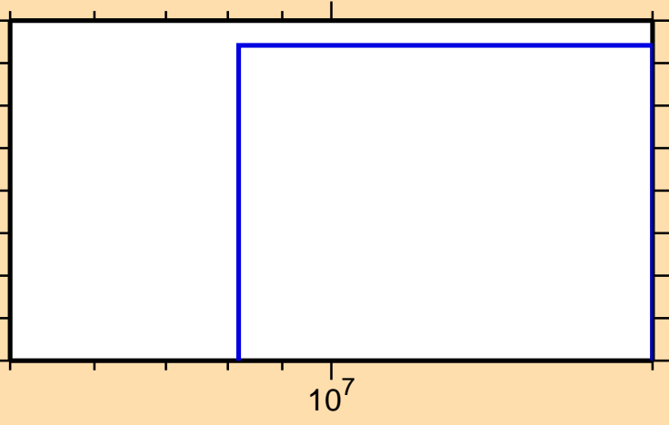
\sigma vs. E for ^{59}\text{Ni}(n,\text{He3})
