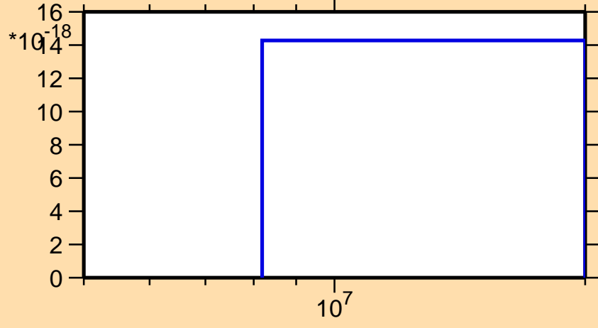
\sigma vs. E for ^{59}\text{Ni}(\text{mt } 45)
