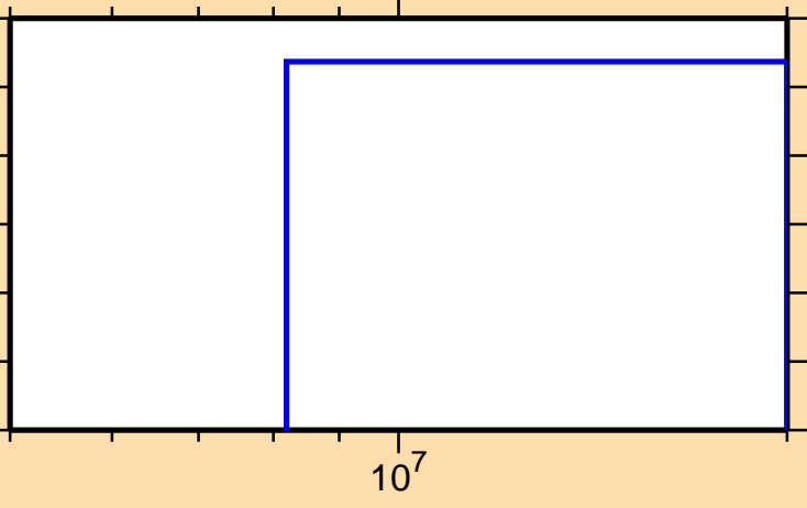
\sigma vs. E for ^{59}\text{Ni}(n,\text{pd})
