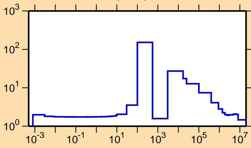
\sigma vs. E for ^{59}\text{Ni}(n,\text{el.})
