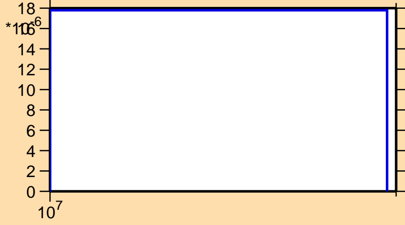
\sigma vs. E for ^{60}\text{Ni}(n,t)
