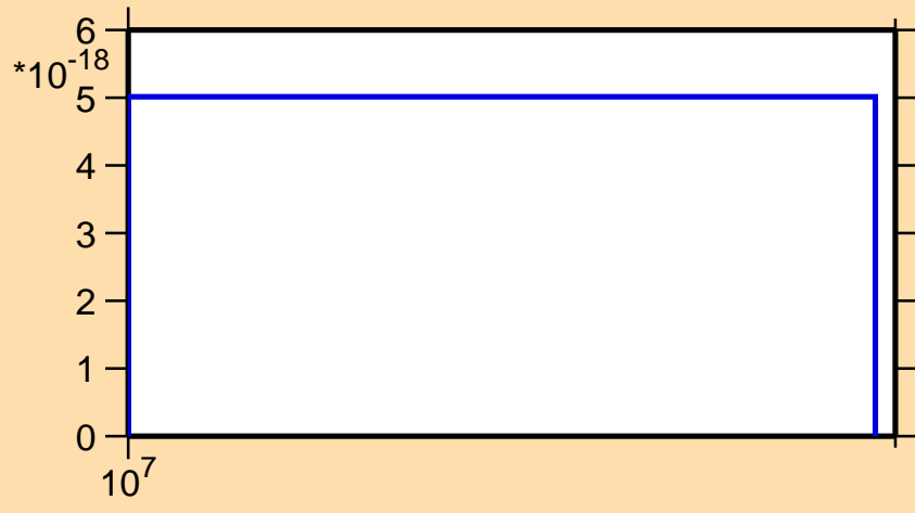
\sigma vs. E for ^{60}\text{Ni}(n,\text{pt})
