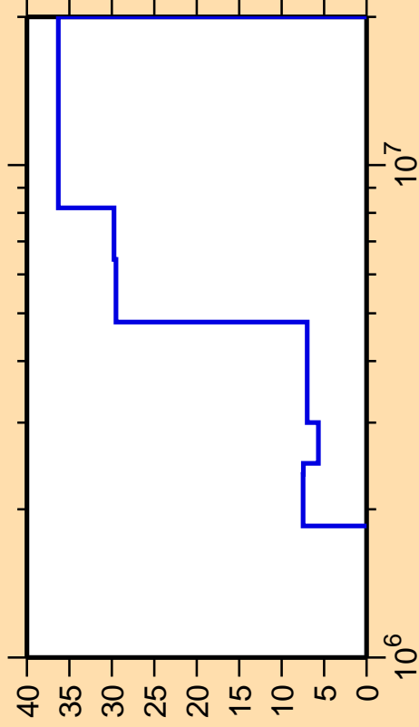
\Delta\sigma/\sigma vs. E for ^{60}\text{Ni}(n,n_2)
