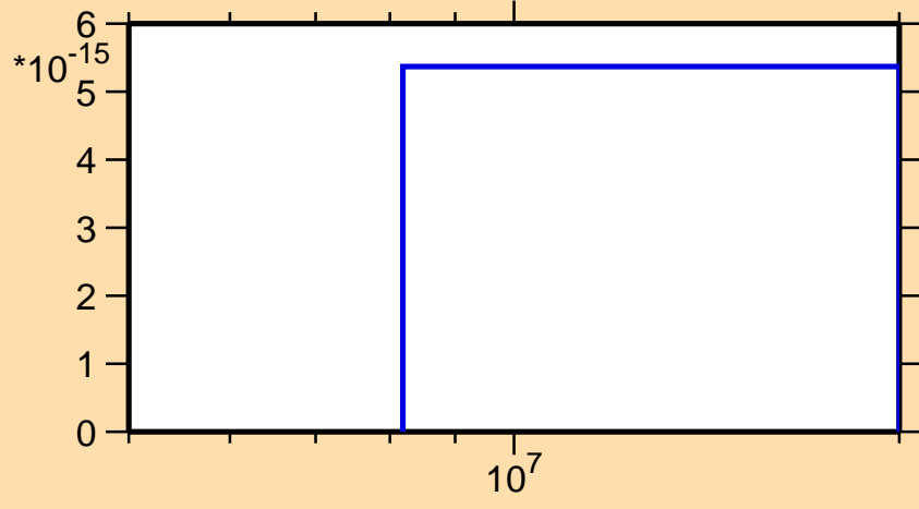
\sigma vs. E for ^{60}\text{Ni}(\text{mt117})
