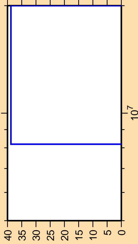
\Delta\sigma/\sigma vs. E for ^{60}\text{Ni}(n,n_1)
