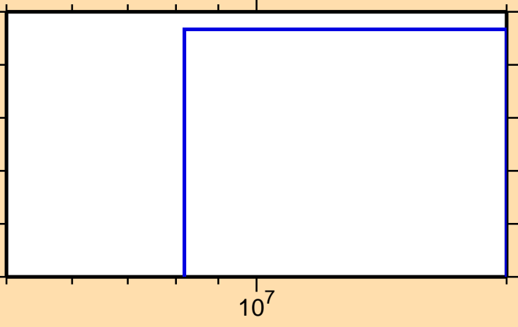
\sigma vs. E for ^{60}\text{Ni}(n,\text{He3})
