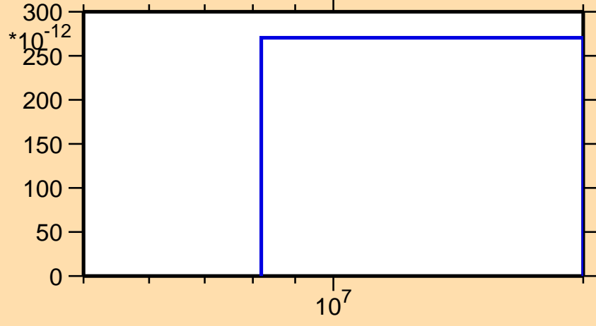
\sigma vs. E for ^{60}\text{Ni}(n,\text{nd})
