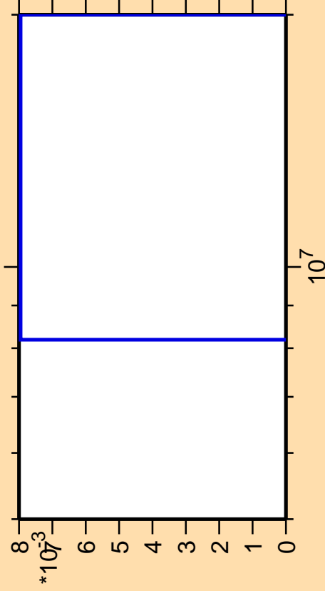
\Delta\sigma/\sigma vs. E for ^{60}\text{Ni}(\text{mt117})
