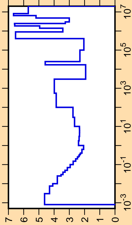
\Delta\sigma/\sigma vs. E for ^{60}\text{Ni}(n,\text{tot.})
