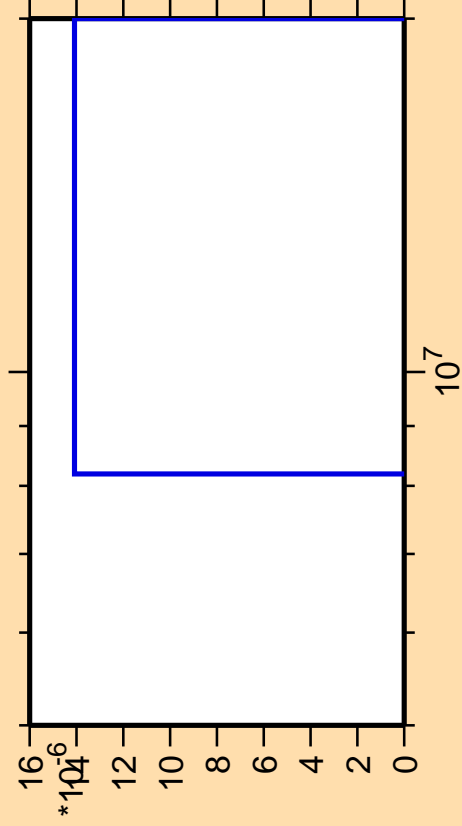
\Delta\sigma/\sigma vs. E for ^{60}\text{Ni}(n,\text{pt})
