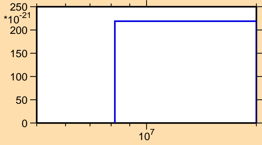
\sigma vs. E for ^{60}\text{Ni} (mt 34)
