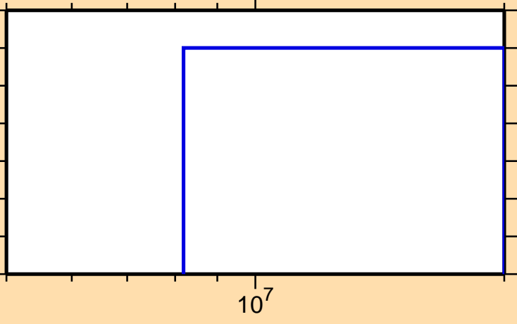
\sigma vs. E for ^{60}\text{Ni}(n,\text{pd})
