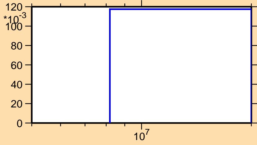
\sigma vs. E for ^{60}\text{Ni}(n,np)
