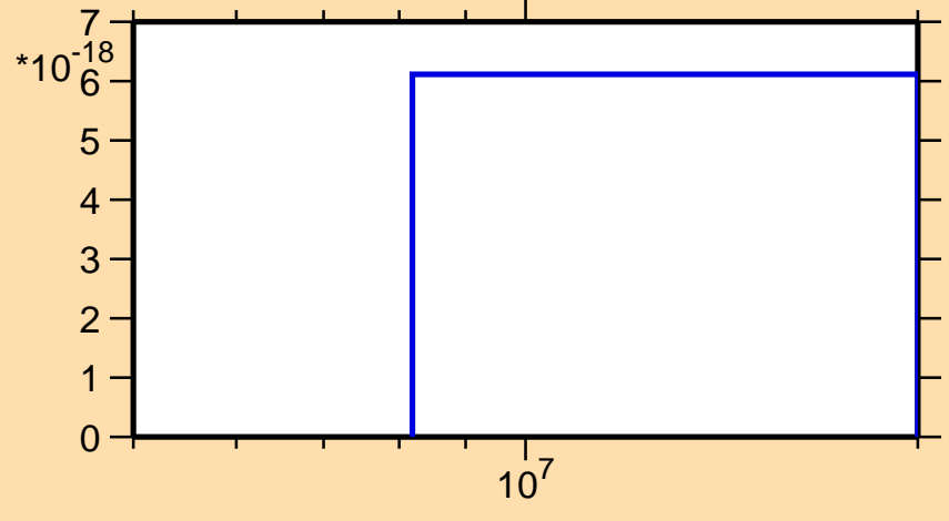
\sigma vs. E for ^{60}\text{Ni}(n,\text{pt})
