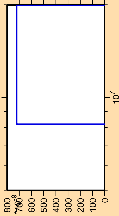
\Delta\sigma/\sigma vs. E for ^{60}\text{Ni} (mt 34)
