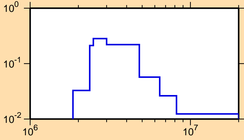
\sigma vs. E for ^{60}\text{Ni}(n,n_2)
