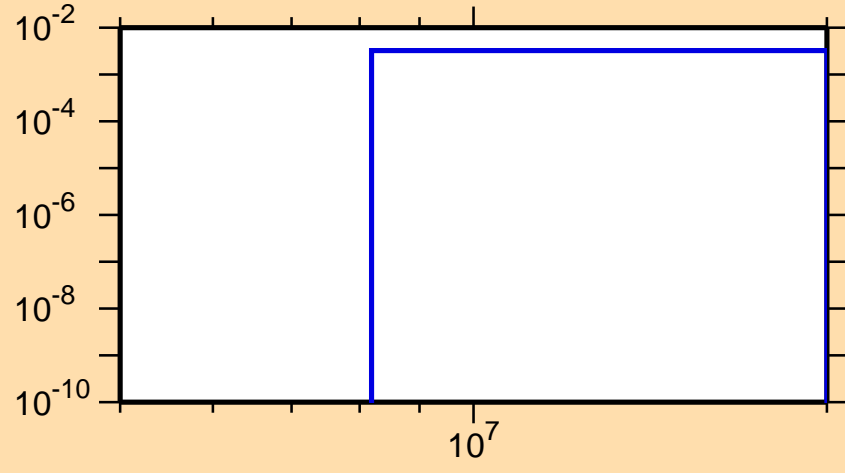
\sigma vs. E for ^{61}\text{Ni}(n,d)
