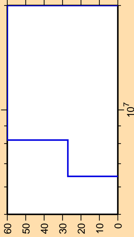
\Delta\sigma/\sigma vs. E for ^{61}\text{Ni}(n,d)
