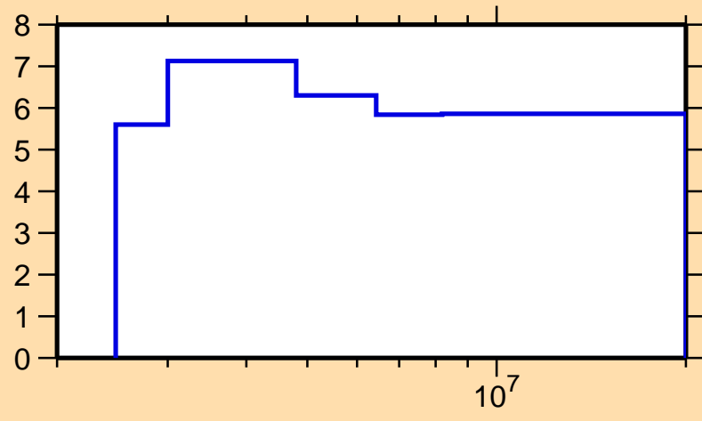
\Delta\sigma/\sigma vs. E for ^{61}\text{Ni}(n,n\text{onel.})
