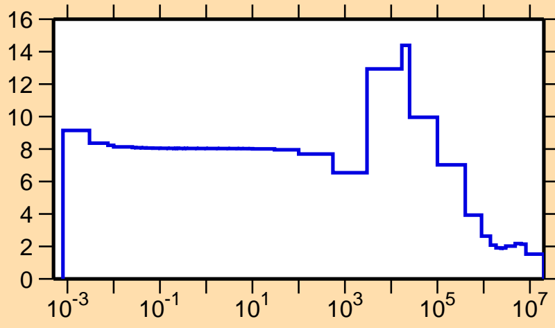
\sigma vs. E for ^{61}\text{Ni}(n,\text{el.})
