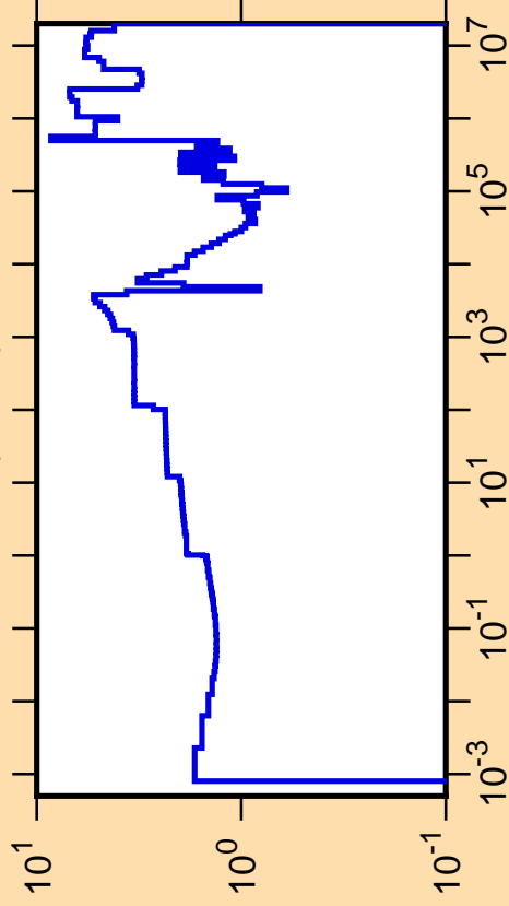
\Delta\sigma/\sigma vs. E for ^{62}\text{Ni}(n,\text{tot.})
