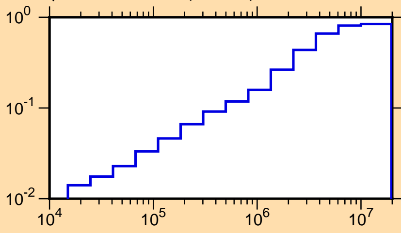
\mu vs. E for ^{62}\text{Ni}(\text{mt251})
