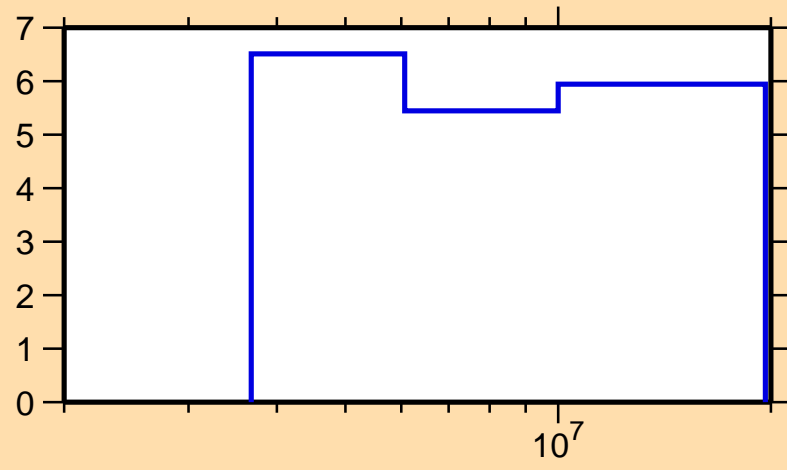
\Delta\sigma/\sigma vs. E for ^{62}\text{Ni}(n,n\text{nonel.})
