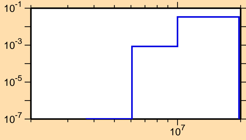
\sigma vs. E for ^{62}\text{Ni}(n,p)
