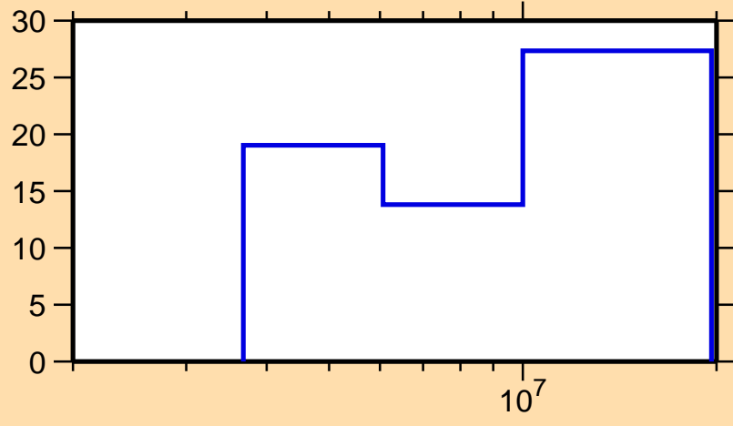
\Delta\sigma/\sigma vs. E for ^{62}\text{Ni}(n,n\text{cont.})
