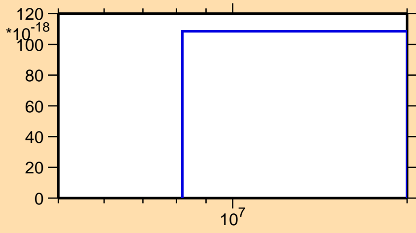
\sigma vs. E for ^{62}\text{Ni}(n,nt)
