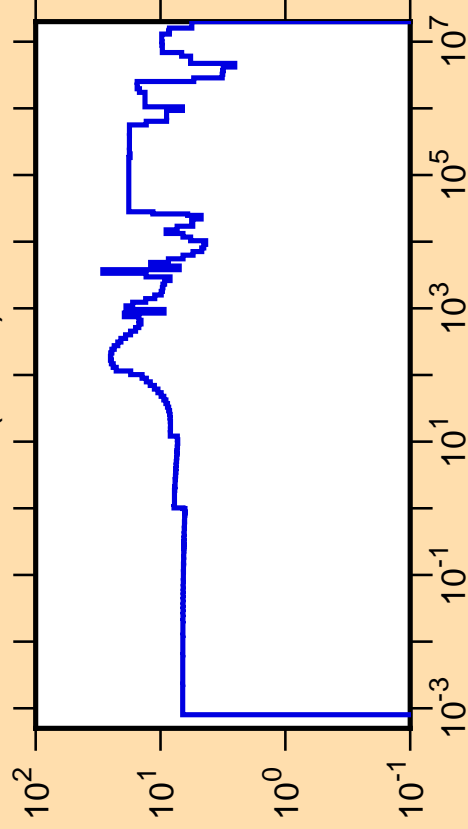
\Delta\sigma/\sigma vs. E for ^{63}\text{Ni}(n,\text{tot.})
