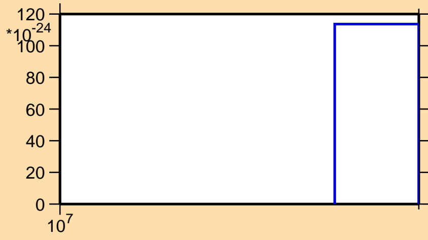
\sigma vs. E for ^{63}\text{Ni}(n,\text{pd})
