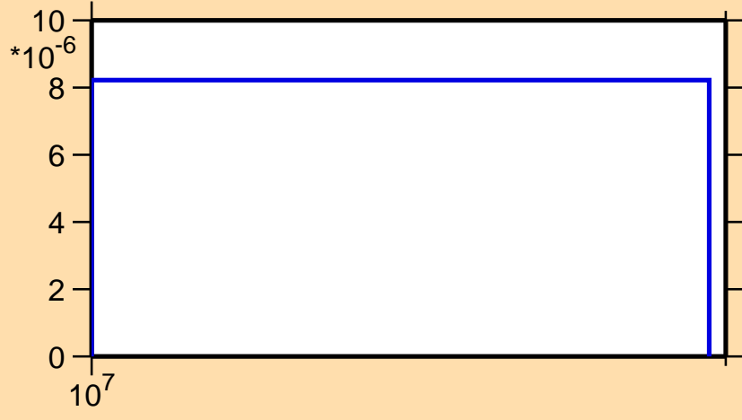
\sigma vs. E for ^{63}\text{Ni}(n,3n)
