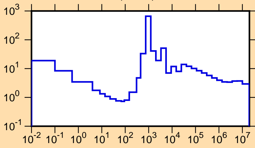
\sigma vs. E for ^{63}\text{Ni}(n,\text{tot.})
