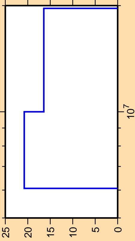
\Delta\sigma/\sigma vs. E for ^{63}\text{Ni}(n,2n)
