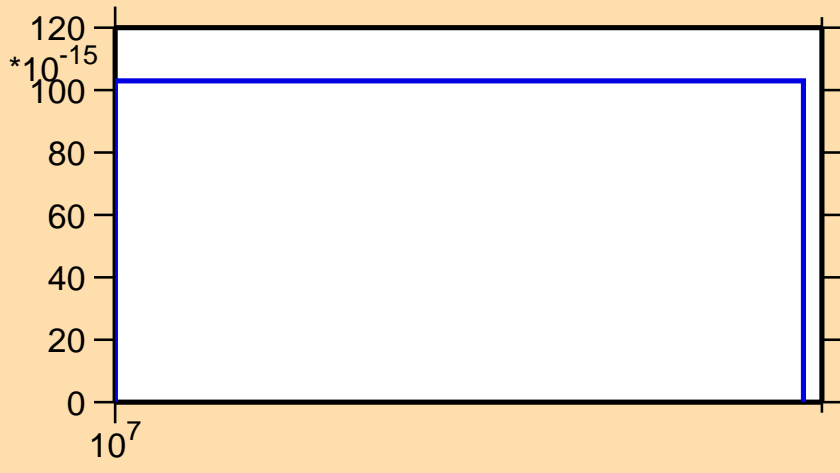
\sigma vs. E for ^{63}\text{Ni}(n,p\alpha)
