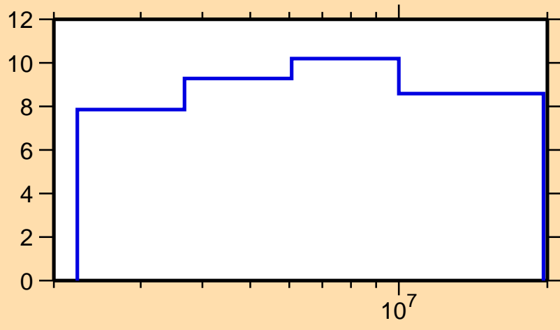
\Delta\sigma/\sigma vs. E for ^{63}\text{Ni}(n,n\text{nonel.})
