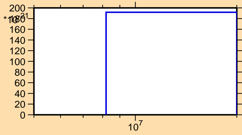
\sigma vs. E for ^{63}\text{Ni}(\text{mt } 34)
