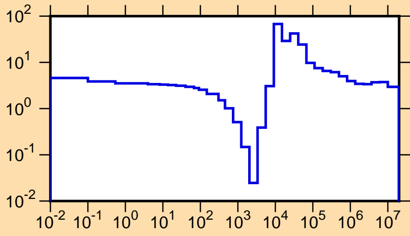
\sigma vs. E for ^{64}\text{Ni}(n,\text{tot.})
