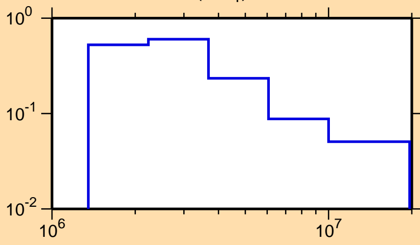
\sigma vs. E for ^{64}\text{Ni}(n,n_1)
