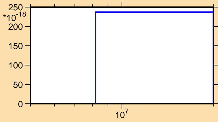
\sigma vs. E for ^{64}\text{Ni}(n,\text{nd})
