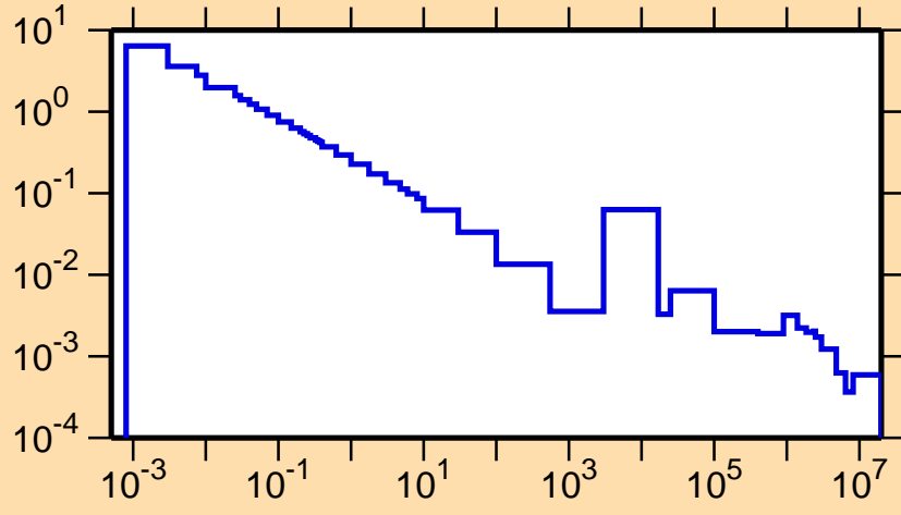
\sigma vs. E for ^{64}\text{Ni}(n,\gamma)
