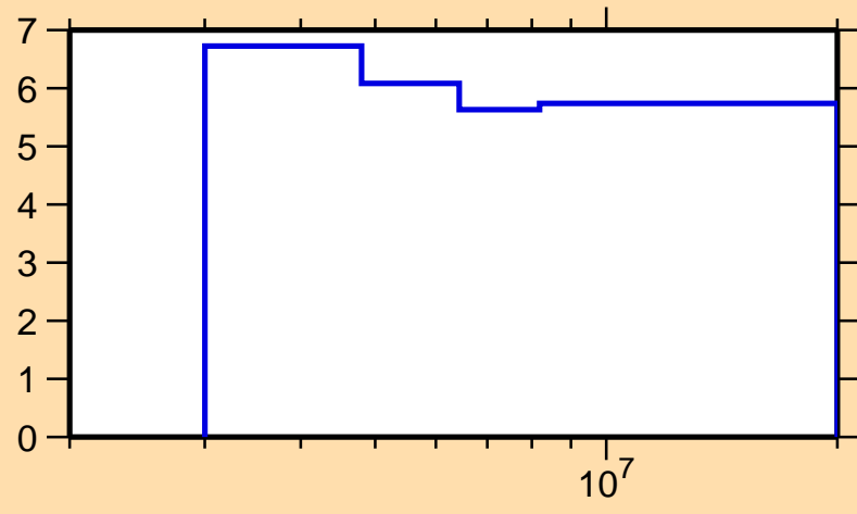
\Delta\sigma/\sigma vs. E for ^{64}\text{Ni}(n,n\text{onel.})
