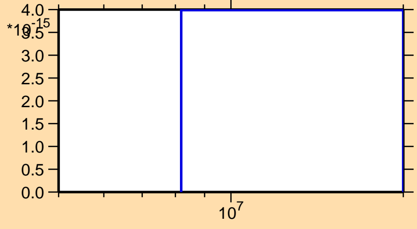
\sigma vs. E for ^{64}\text{Ni}(n,\text{nt})
