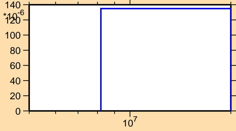
\sigma vs. E for ^{64}\text{Ni}(n,d)
