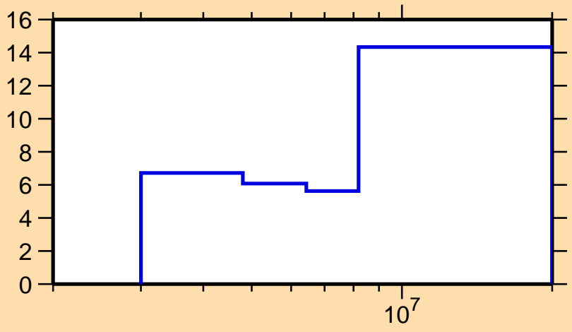
\Delta\sigma/\sigma vs. E for ^{64}\text{Ni}(n,\text{inel.})
