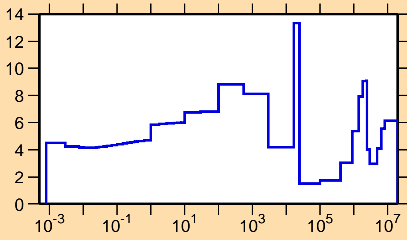
\Delta\sigma/\sigma vs. E for ^{64}\text{Ni}(n,\text{tot.})
