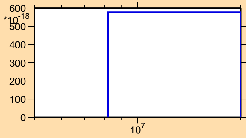
\sigma vs. E for ^{64}\text{Ni}(n,\text{He3})
