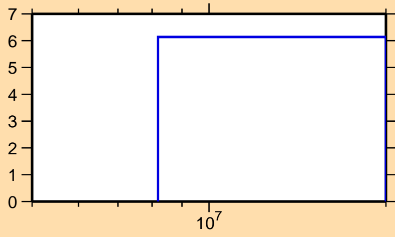
\Delta\sigma/\sigma vs. E for ^{64}\text{Ni}(n,\text{tot.})
