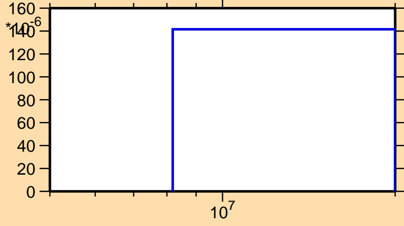
\sigma vs. E for ^{64}\text{Ni}(n,np)
