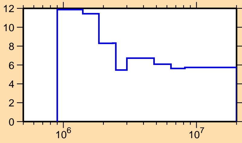
\Delta\sigma/\sigma vs. E for ^{64}\text{Ni}(n,\text{nonel.})
