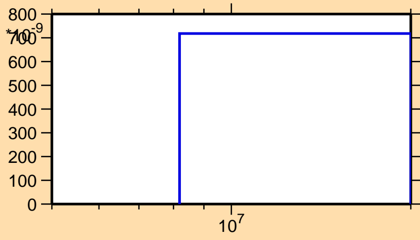
\sigma vs. E for ^{64}\text{Ni}(n,t)
