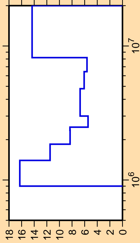
\Delta\sigma/\sigma vs. E for ^{64}\text{Ni}(n,\text{inel.})
