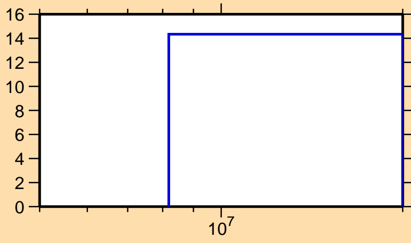
\Delta\sigma/\sigma vs. E for ^{64}\text{Ni}(n,\text{inel.})
