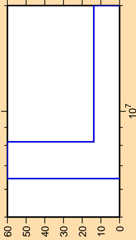
\Delta\sigma/\sigma vs. E for ^{64}\text{Ni}(n,\alpha)
