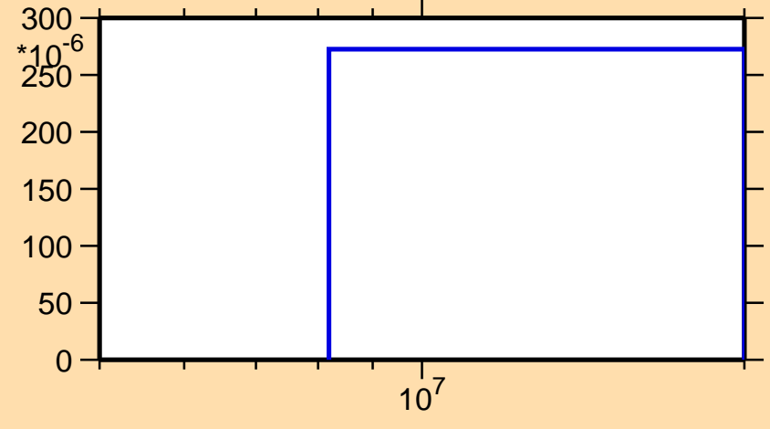
\sigma vs. E for ^{64}\text{Ni}(n,n\alpha)
