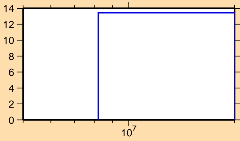
\Delta\sigma/\sigma vs. E for ^{64}\text{Ni}(n,2n)
