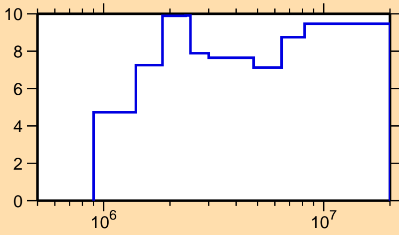
\Delta\sigma/\sigma vs. E for ^{64}\text{Ni}(n,\text{el.})
