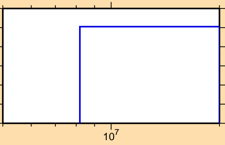
\sigma vs. E for ^{64}\text{Ni}(n,3n)
