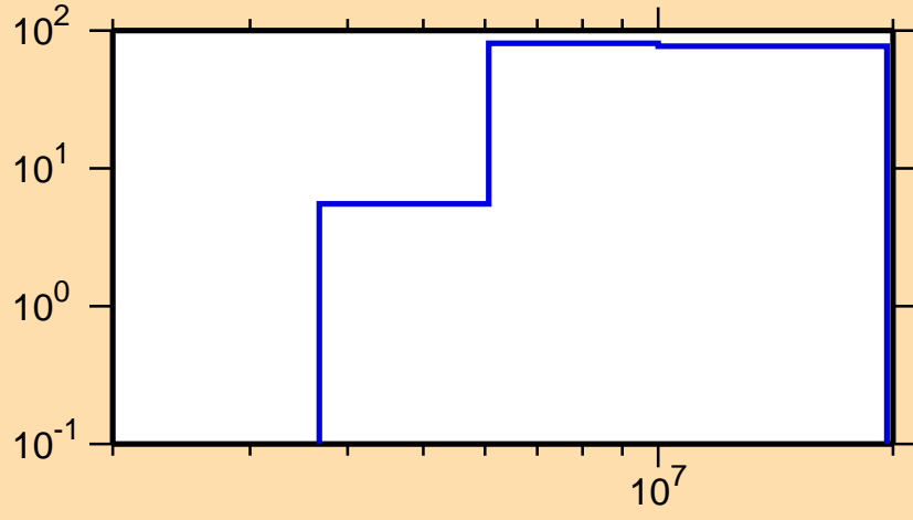
\Delta\sigma/\sigma vs. E for ^{65}\text{Ni}(n,p)
