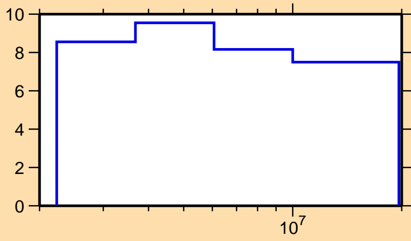
\Delta\sigma/\sigma vs. E for ^{65}\text{Ni}(n,n\text{onel.})
