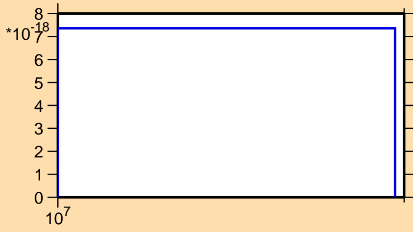
\sigma vs. E for ^{65}\text{Ni}(n,nt)
