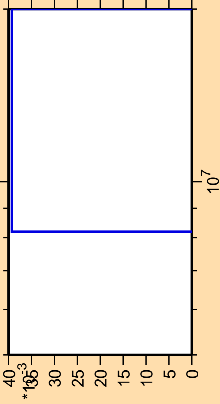
\Delta\sigma/\sigma vs. E for ^{65}\text{Ni}(n,2np)
