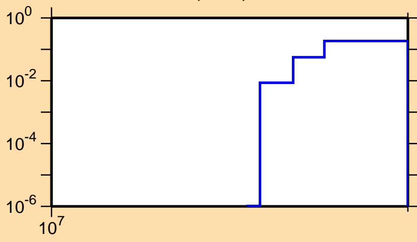
\sigma vs. E for ^{67}\text{Ni}(n,3n)
