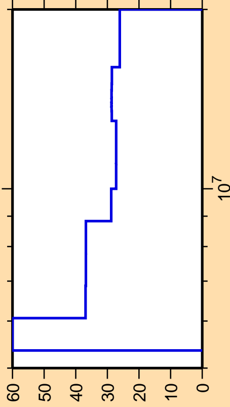
\Delta\sigma/\sigma vs. E for ^{67}\text{Ni}(n,2n)
