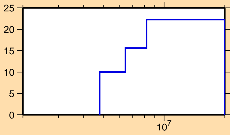
\Delta\sigma/\sigma vs. E for ^{67}\text{Ni}(n,\text{tot.})
