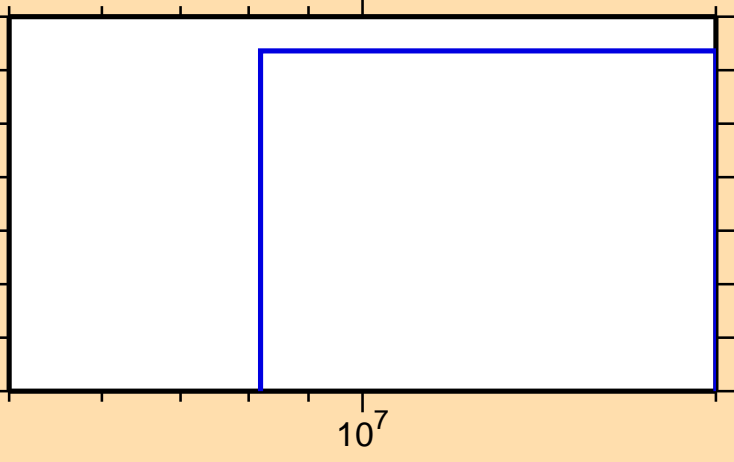
\sigma vs. E for ^{67}\text{Ni}(n,t)
