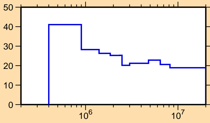
\Delta\sigma/\sigma vs. E for ^{67}\text{Ni}(n,\text{nonel.})
