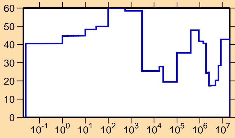
\Delta\sigma/\sigma vs. E for ^{67}\text{Ni}(n,\text{el.})
