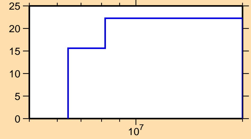
\Delta\sigma/\sigma vs. E for ^{67}\text{Ni}(n,\text{tot.})
