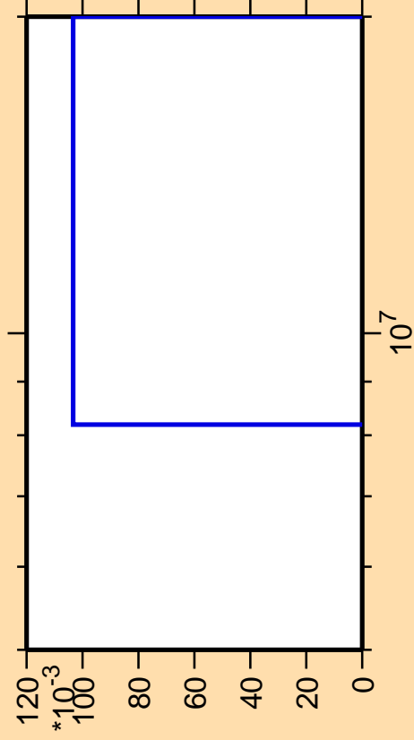
\Delta\sigma/\sigma vs. E for ^{67}\text{Ni}(n,2n\alpha)
