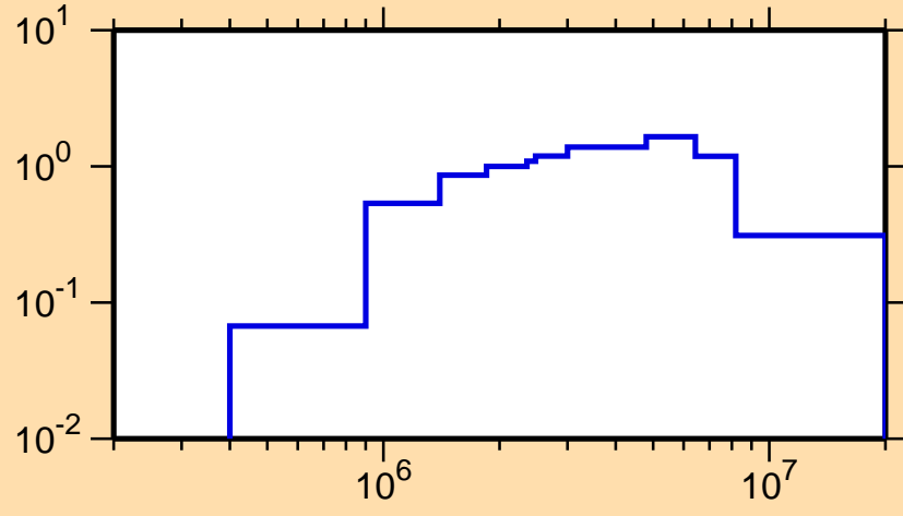
\sigma vs. E for ^{67}\text{Ni}(n,\text{inel.})
