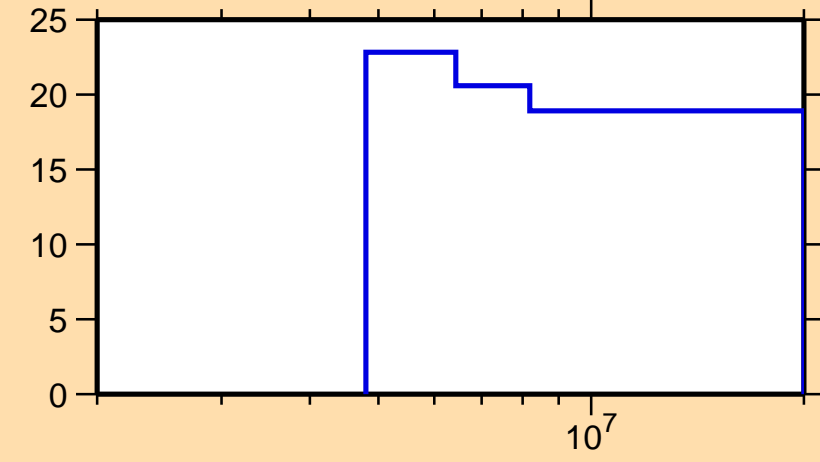
\Delta\sigma/\sigma vs. E for ^{67}\text{Ni}(n,\text{none})
