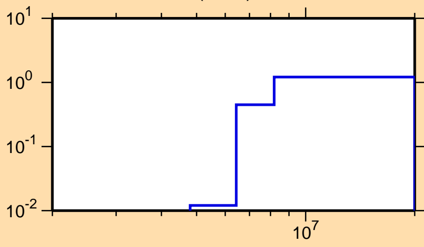
\sigma vs. E for ^{67}\text{Ni}(n,2n)
