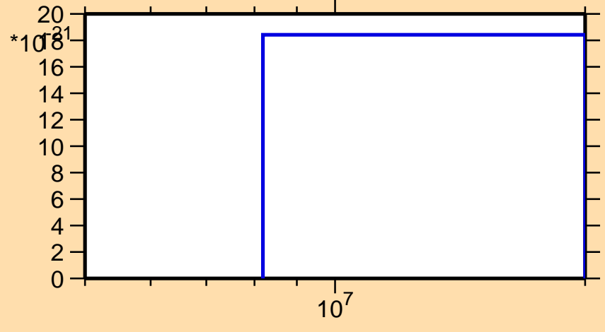
\sigma vs. E for ^{67}\text{Ni}(n,nt)
