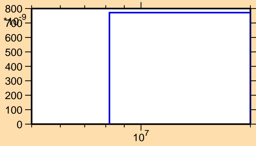
\sigma vs. E for ^{67}\text{Ni}(n,np)
