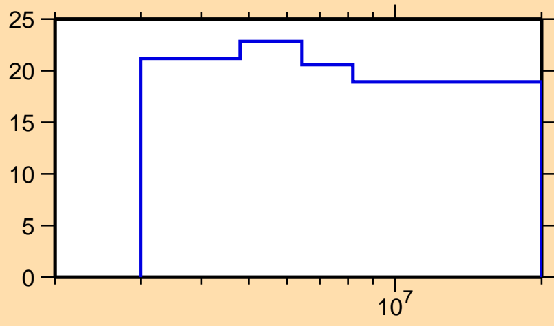
\Delta\sigma/\sigma vs. E for ^{67}\text{Ni}(n,n\text{onel.})
