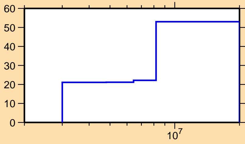
\Delta\sigma/\sigma vs. E for ^{67}\text{Ni}(n,\text{inel.})
