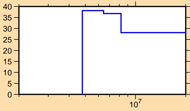
\Delta\sigma/\sigma vs. E for ^{67}\text{Ni}(n,2n)
