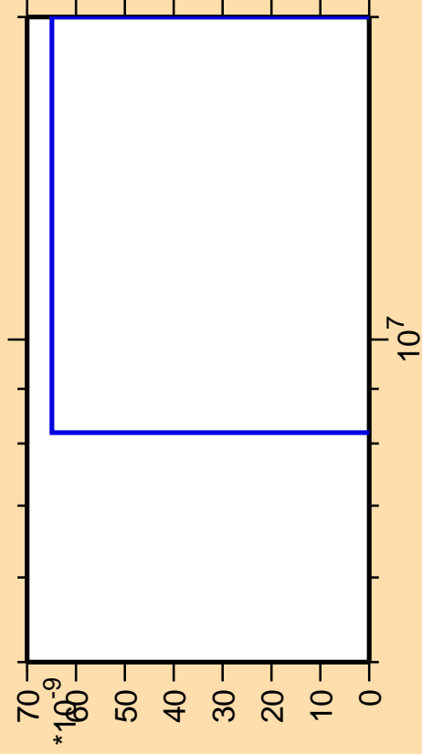
\Delta\sigma/\sigma vs. E for ^{67}\text{Ni}(n,nt)
