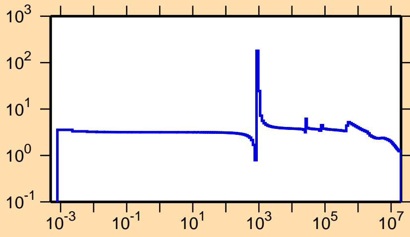
\sigma vs. E for ^{68}\text{Ni}(n,\text{el.})
