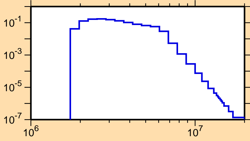
\sigma vs. E for ^{68}\text{Ni}(n,n_1)
