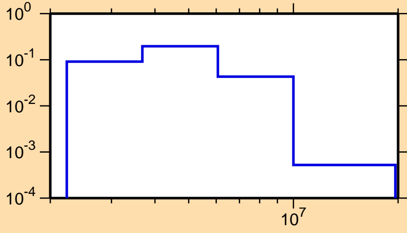
\sigma vs. E for ^{68}\text{Ni}(n,n_4)
