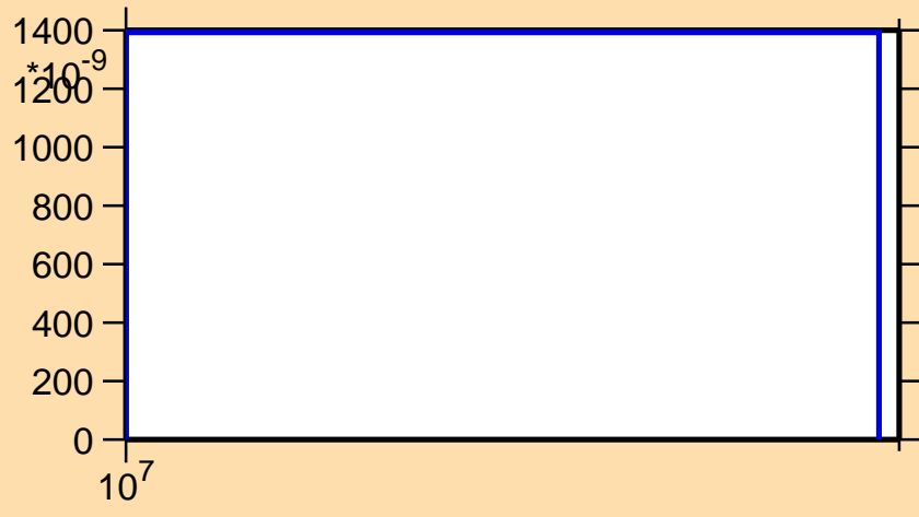
\sigma vs. E for ^{68}\text{Ni}(n,d)
