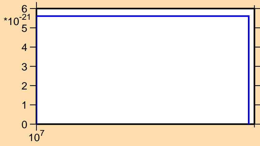
\sigma vs. E for ^{68}\text{Ni}(n,2n\alpha)
