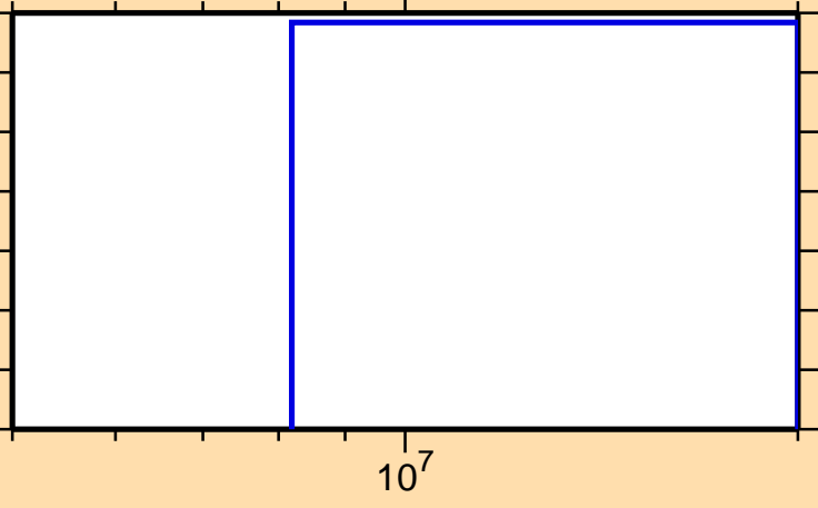
\sigma vs. E for ^{68}\text{Ni}(n,3n)
