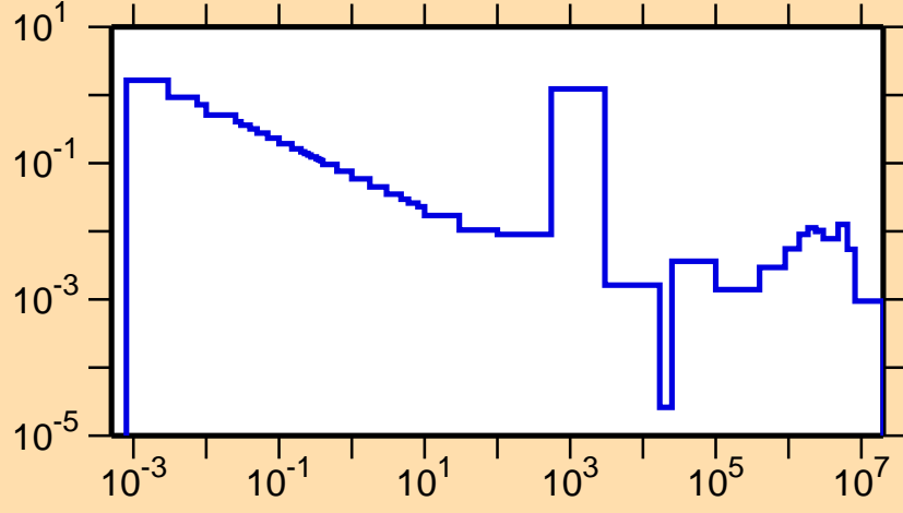
\sigma vs. E for ^{68}\text{Ni}(n,\gamma)
