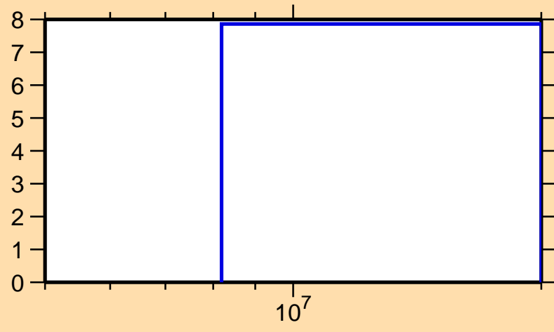
\Delta\sigma/\sigma vs. E for ^{68}\text{Ni}(n,\text{tot.})
