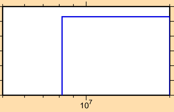
\sigma vs. E for ^{68}\text{Ni}(n,n\alpha)
