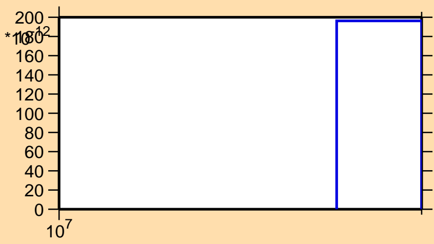
\sigma vs. E for ^{69}\text{Ni}(n,\text{nd})
