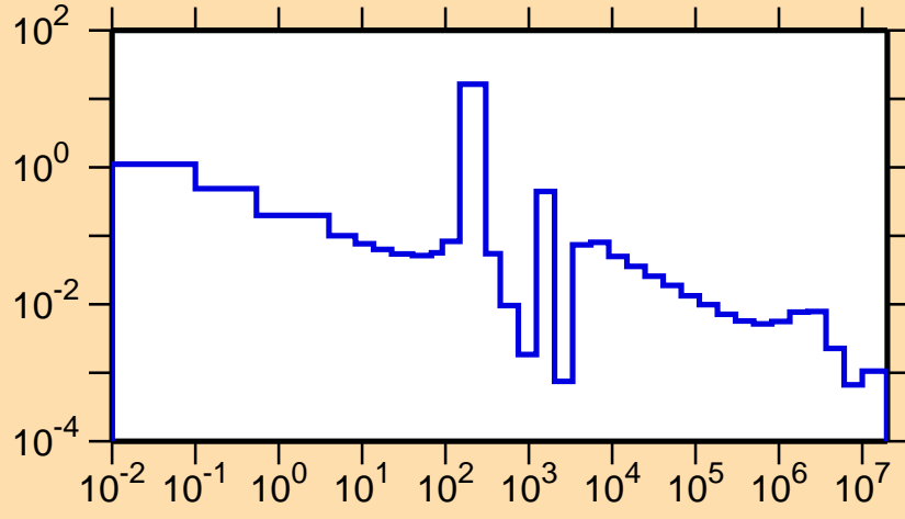
\sigma vs. E for ^{69}\text{Ni}(n,\gamma)
