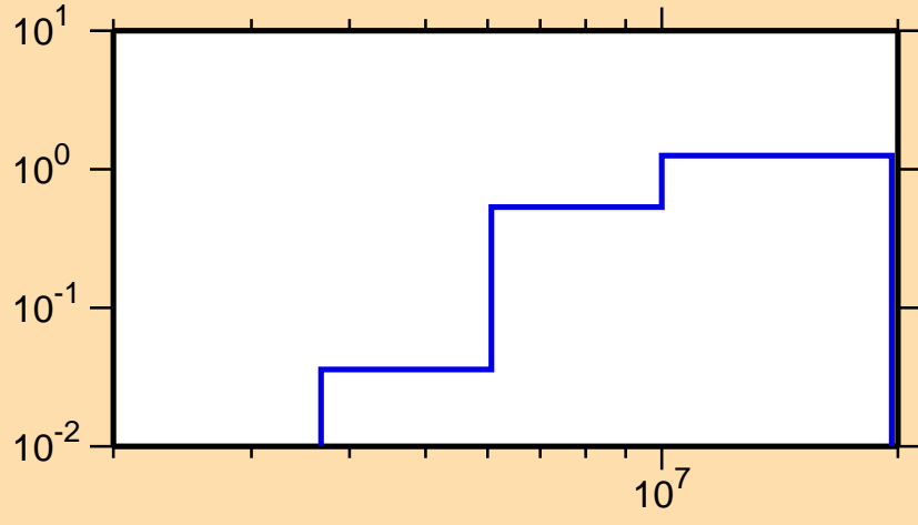
\sigma vs. E for ^{69}\text{Ni}(n,2n)
