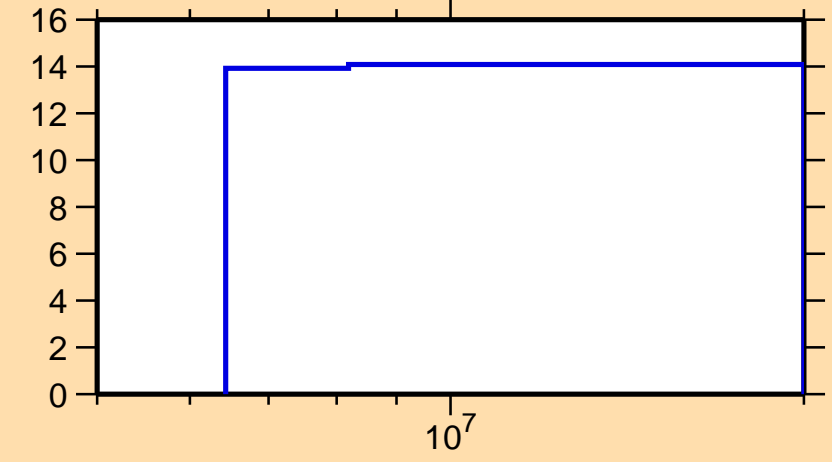
\Delta\sigma/\sigma vs. E for ^{69}\text{Ni}(n,\text{tot.})
