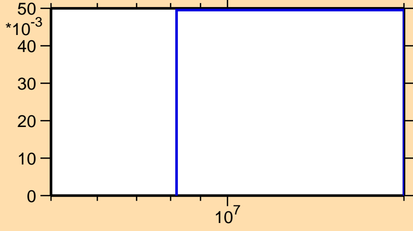
\sigma vs. E for ^{69}\text{Ni}(n,3n)
