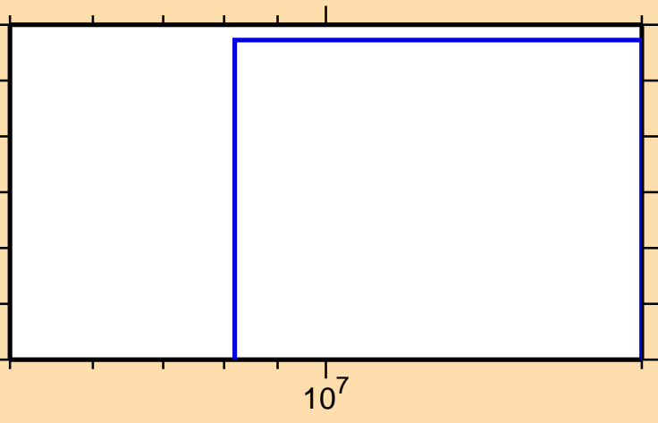
\sigma vs. E for ^{69}\text{Ni}(n,t)
