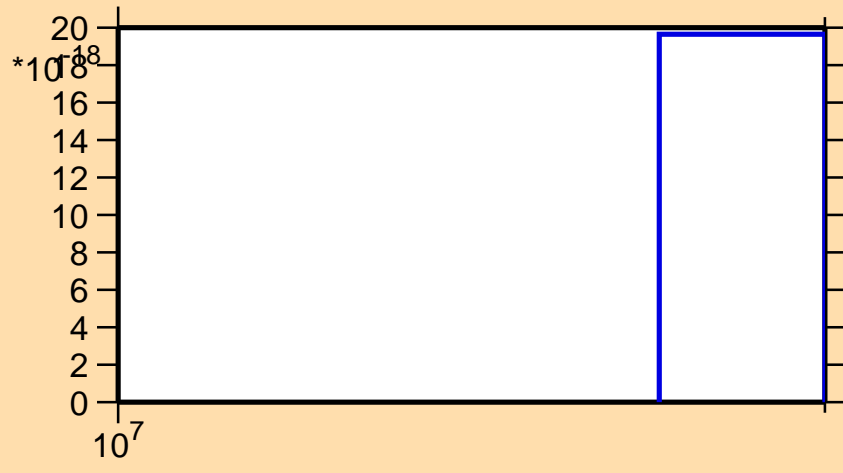
\sigma vs. E for ^{70}\text{Ni}(n,nt)
