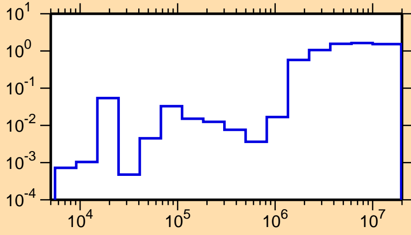
\sigma vs. E for ^{70}\text{Ni}(n,\text{nonel.})
