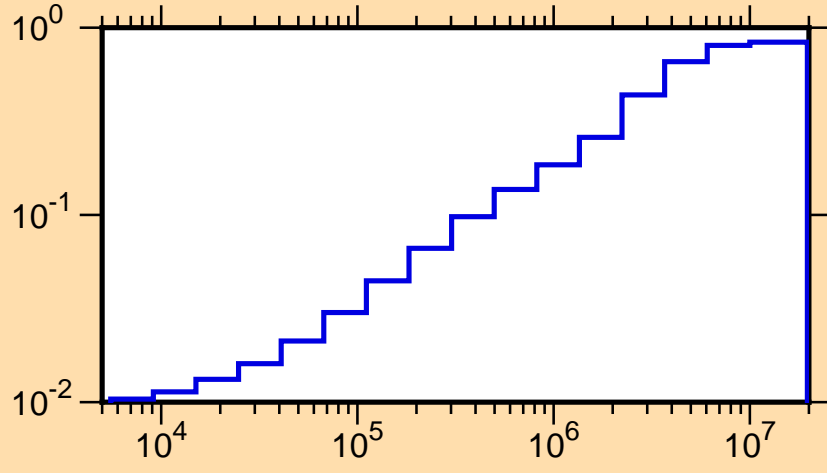
\mu vs. E for ^{71}\text{Ni}(\text{mt251})
