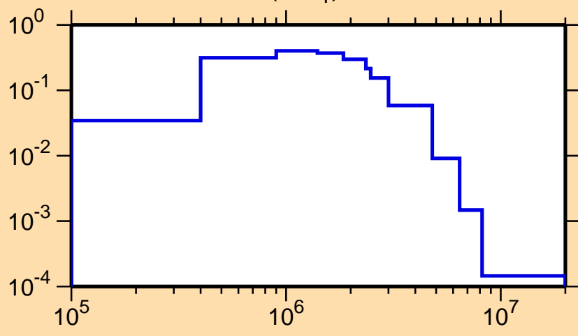
\sigma vs. E for ^{71}\text{Ni}(n,n_1)
