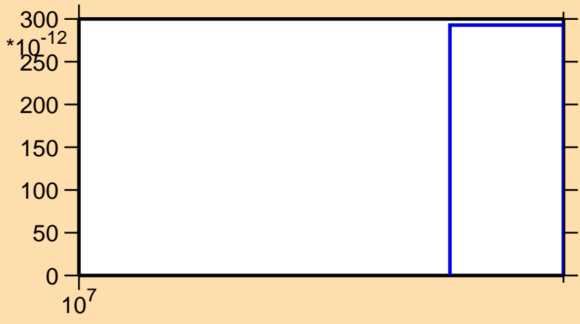
\sigma vs. E for ^{71}\text{Ni}(n,nd)
