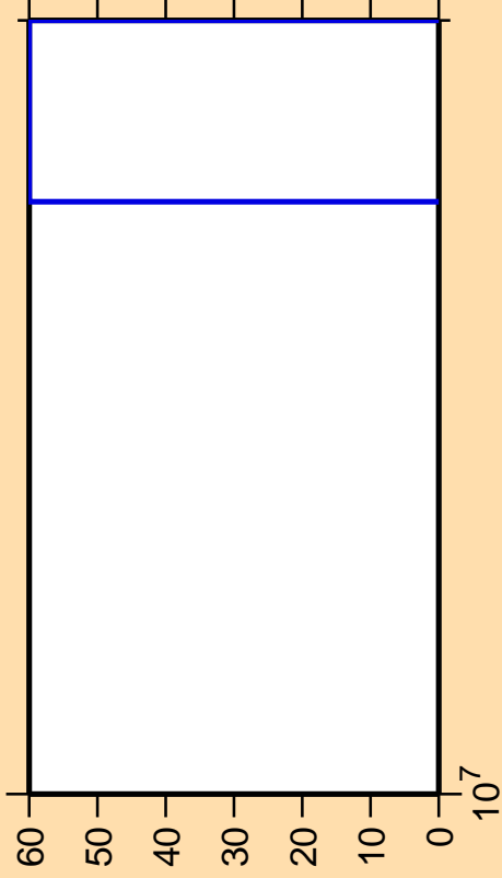
\Delta\sigma/\sigma vs. E for ^{71}\text{Ni}(n,nd)
