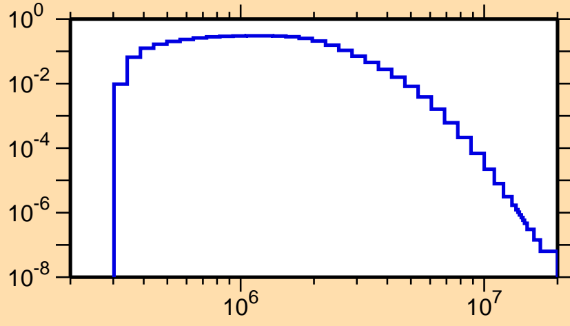
\sigma vs. E for ^{71}\text{Ni}(n,n_3)
