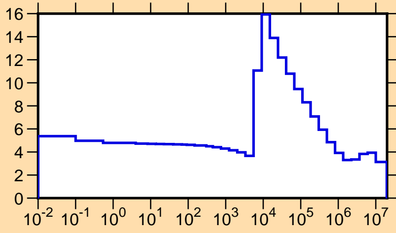
\sigma vs. E for ^{71}\text{Ni}(n,\text{tot.})
