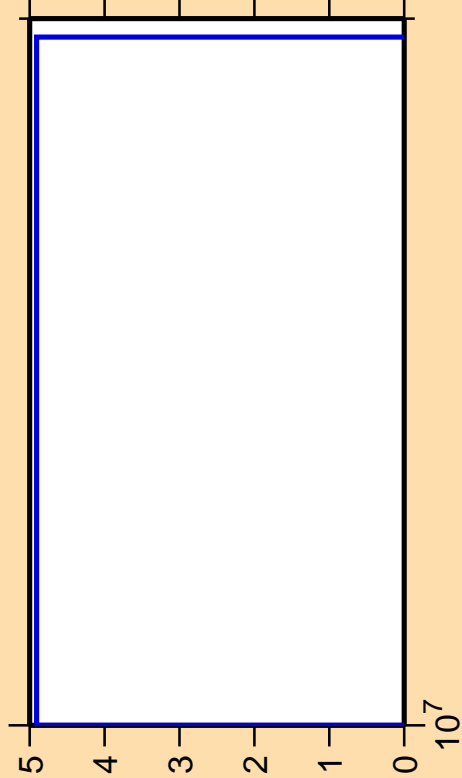
\Delta\sigma/\sigma vs. E for ^{71}\text{Ni}(n,nt)
