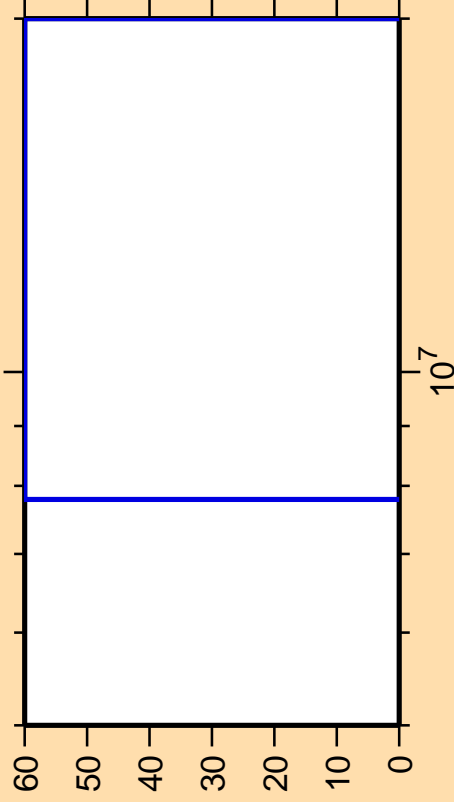
\Delta\sigma/\sigma vs. E for ^{252}\text{No}(n,2n)
