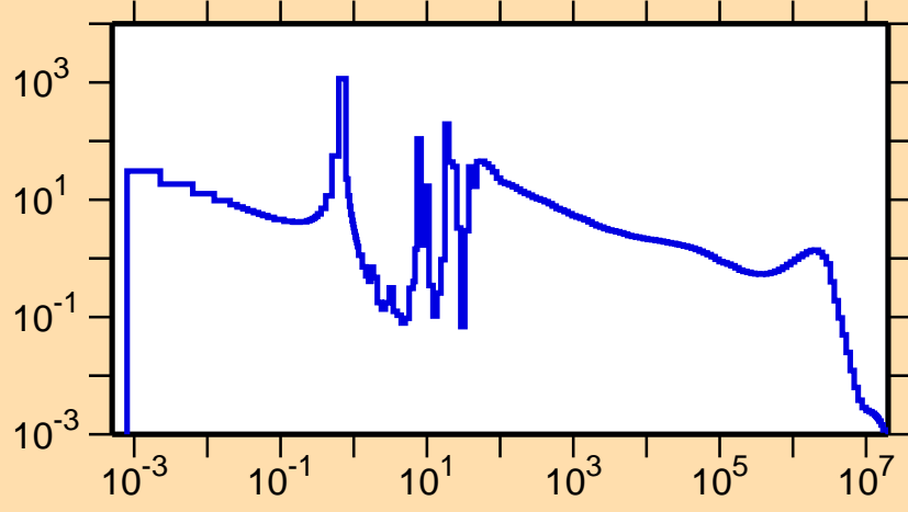
\sigma vs. E for ^{252}\text{No}(n,\gamma)
