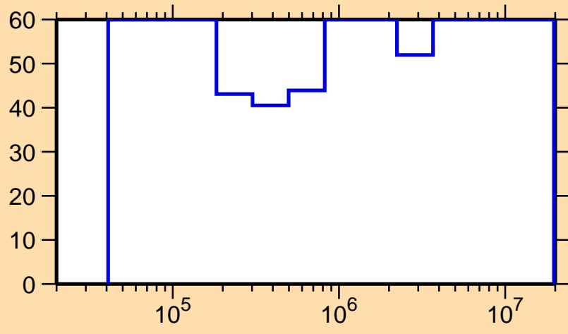
\Delta\sigma/\sigma vs. E for ^{252}\text{No}(n,n_1)
