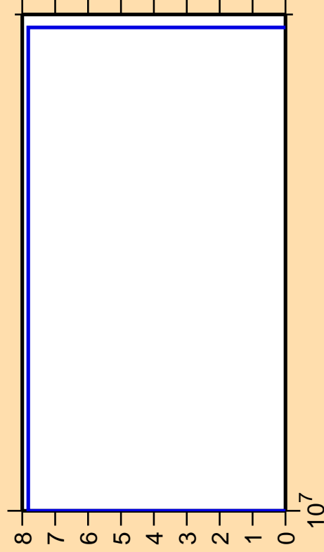
\Delta\sigma/\sigma vs. E for ^{252}\text{No}(\text{mt117})
