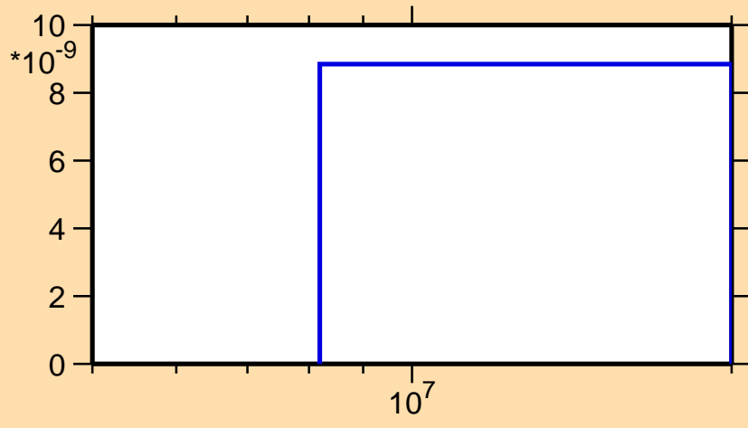
\sigma vs. E for ^{252}\text{No}(n,\text{nd})
