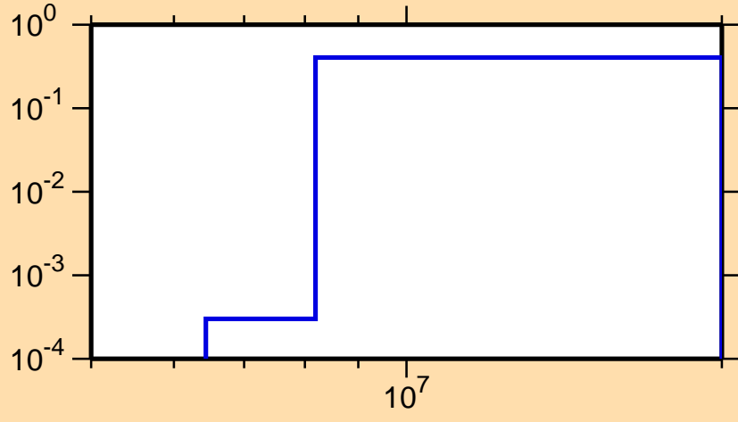
\sigma vs. E for ^{252}\text{No}(n,2n)
