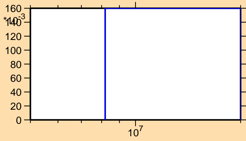
\sigma vs. E for ^{252}\text{No}(n,2n\alpha)
