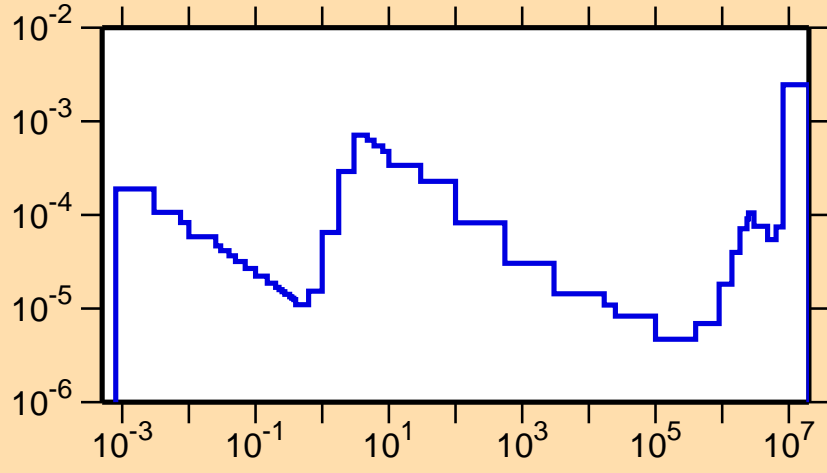
\sigma vs. E for ^{252}\text{No}(n,\alpha)
