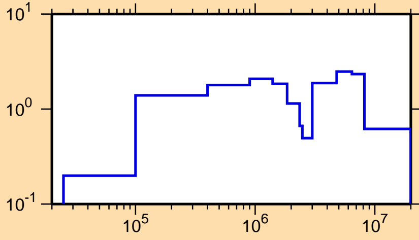
\sigma vs. E for ^{252}\text{No}(n,\text{inel.})
