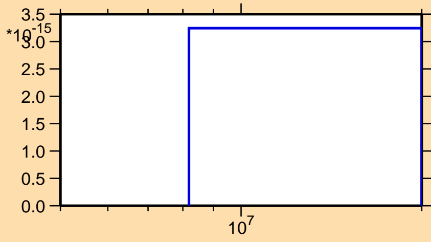
\sigma vs. E for ^{252}\text{No}(n,\text{pt})
