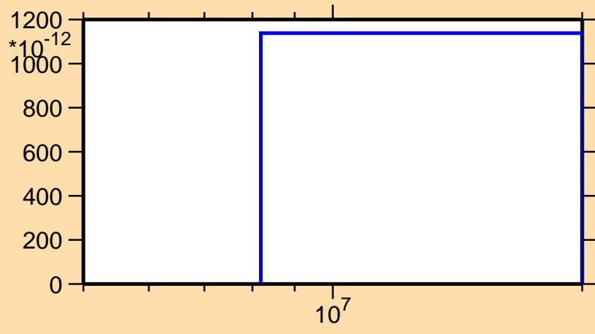
\sigma vs. E for ^{252}\text{No}(n,\text{He3})
