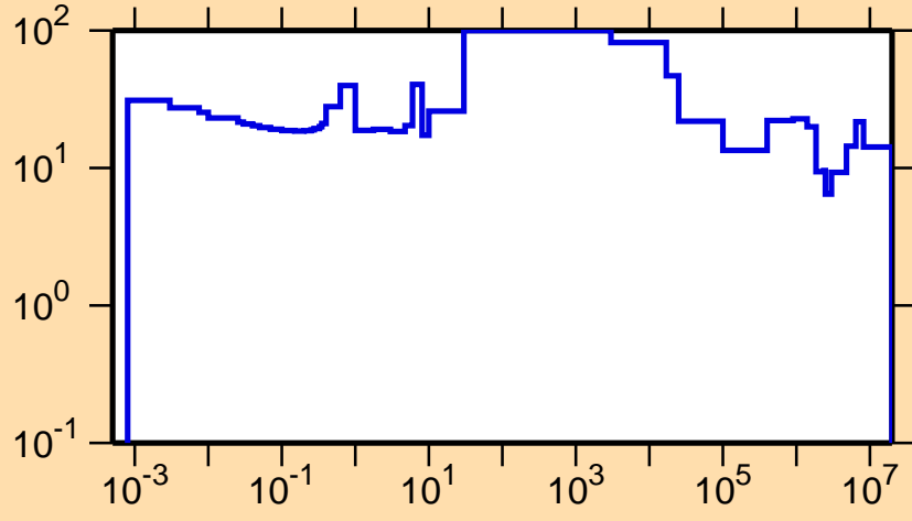
\Delta\sigma/\sigma vs. E for ^{252}\text{No}(n,tot.)
