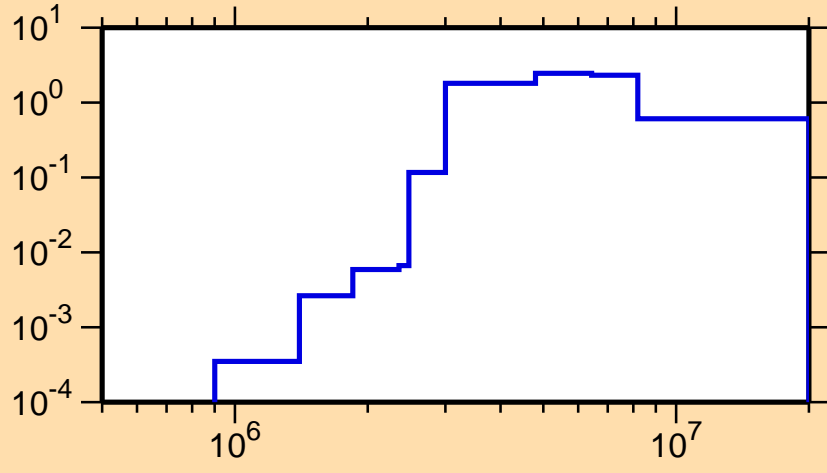
\sigma vs. E for ^{252}\text{No}(n,n\text{cont.})
