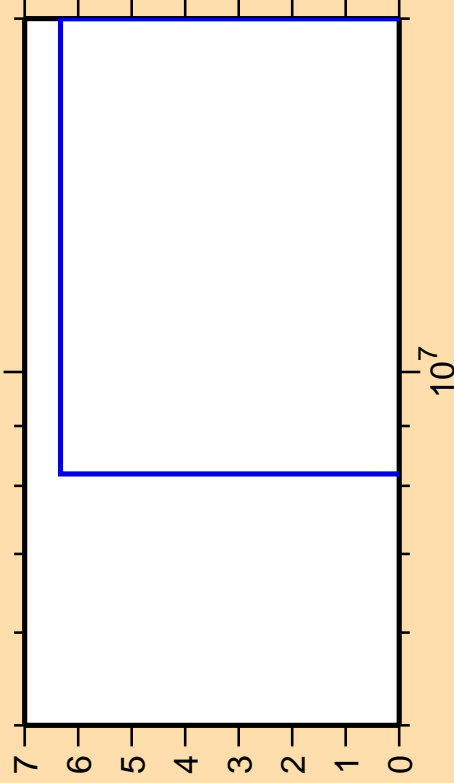
\Delta\sigma/\sigma vs. E for ^{252}\text{No}(\text{mt117})
