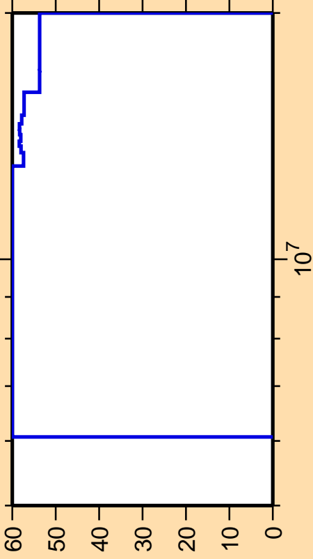
\Delta\sigma/\sigma vs. E for ^{253}\text{No}(n,n\text{cont.})
