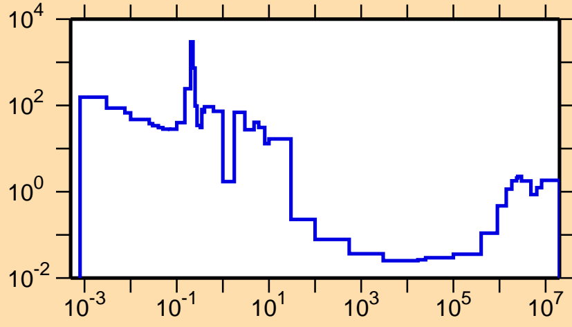
\sigma vs. E for ^{253}\text{No}(n,f)
