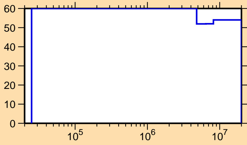
\Delta\sigma/\sigma vs. E for ^{253}\text{No}(n,n_1)
