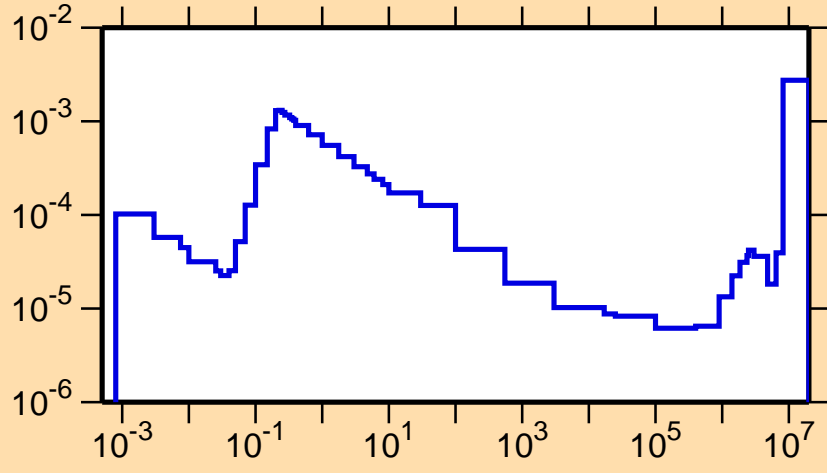
\sigma vs. E for ^{253}\text{No}(n,\alpha)
