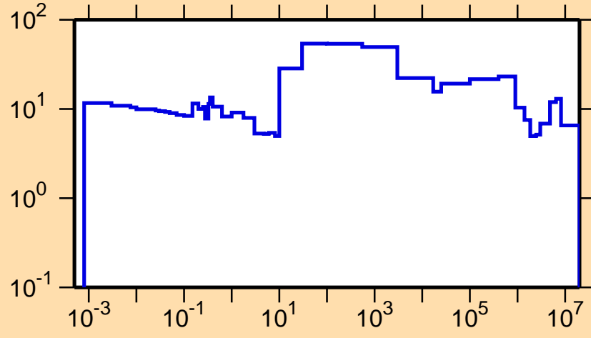
\Delta\sigma/\sigma vs. E for ^{253}\text{No}(n,tot.)
