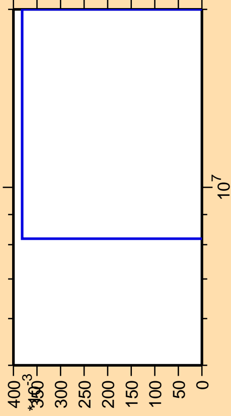
\Delta\sigma/\sigma vs. E for ^{253}\text{No}(\text{mt } 34)
