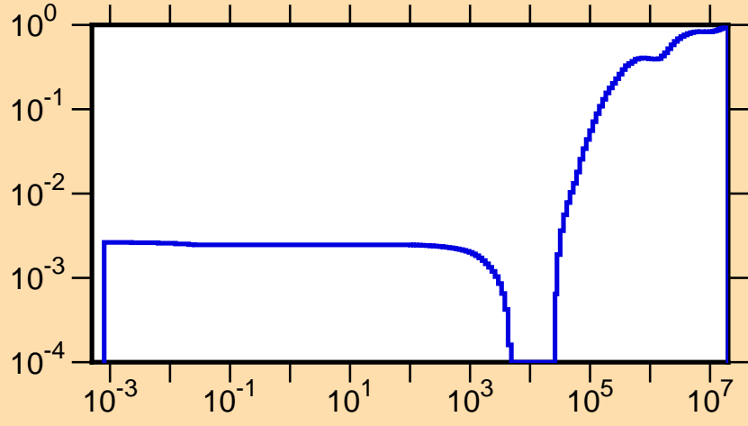
\mu vs. E for ^{254}\text{No}(\text{mt251})
