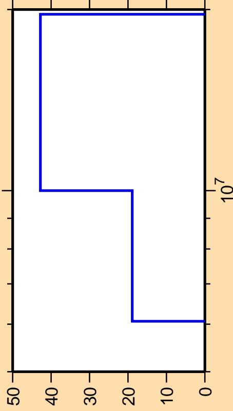
\Delta\sigma/\sigma vs. E for ^{254}\text{No}(n,t)
