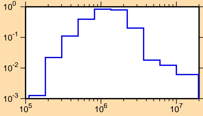
\sigma vs. E for ^{254}\text{No}(n,n_2)
