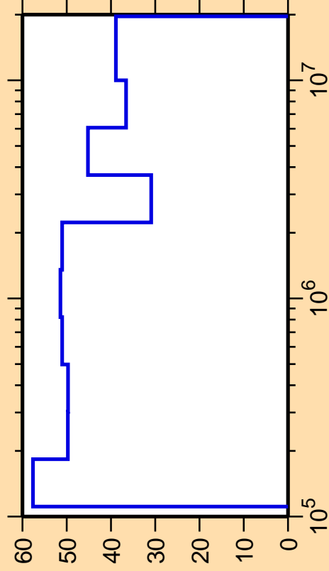
\Delta\sigma/\sigma vs. E for ^{254}\text{No}(n,n_2)
