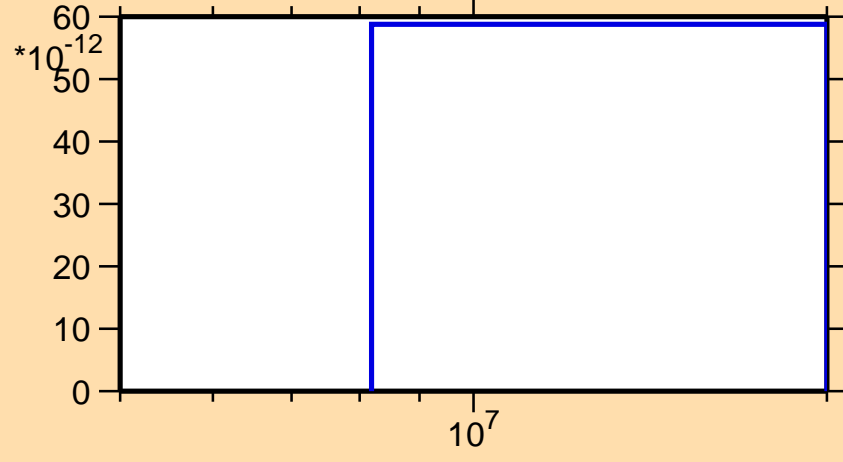
\sigma vs. E for ^{254}\text{No}(n,3n\alpha)
