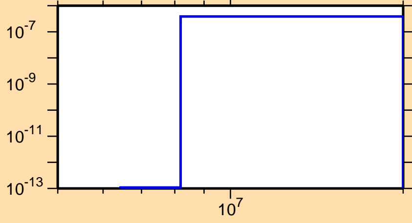
\sigma vs. E for ^{254}\text{No}(n,2n\alpha)
