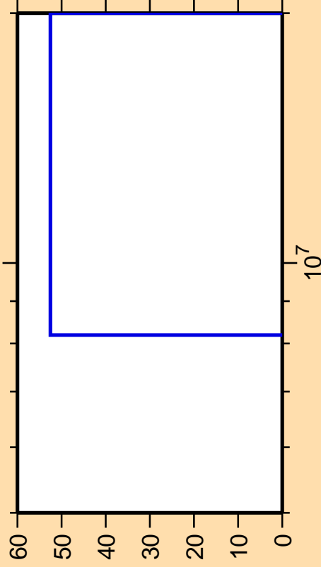
\Delta\sigma/\sigma vs. E for ^{254}\text{No}(n,3n\alpha)
