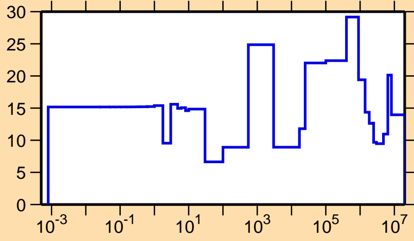
\Delta\sigma/\sigma vs. E for ^{254}\text{No}(n,el.)
