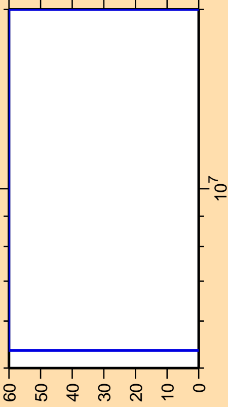
\Delta\sigma/\sigma vs. E for ^{255}\text{No}(n,n\text{cont.})
