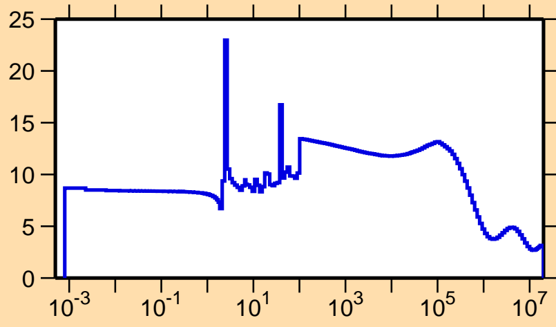
\sigma vs. E for ^{255}\text{No}(n,\text{el.})
