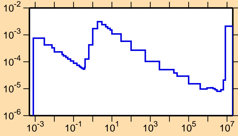
\sigma vs. E for ^{255}\text{No}(n,\alpha)
