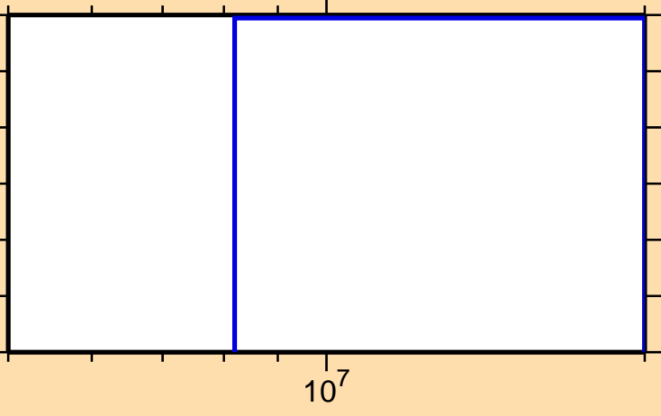
\sigma vs. E for ^{255}\text{No}(n,2np)
