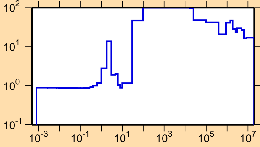
\Delta\sigma/\sigma vs. E for ^{255}\text{No}(n,el.)
