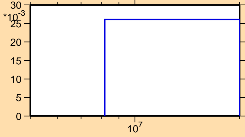
\sigma vs. E for ^{255}\text{No}(n,3n)
