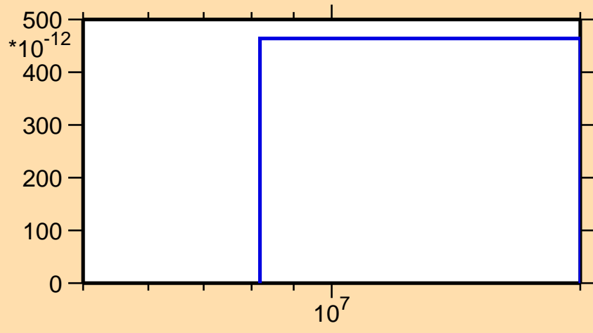
\sigma vs. E for ^{255}\text{No}(n,\text{He}3)
