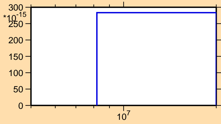
\sigma vs. E for ^{255}\text{No}(\text{mt } 34)
