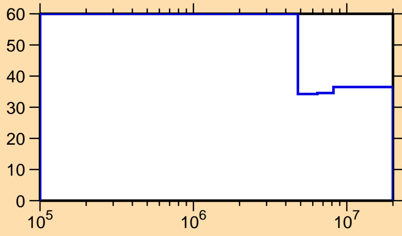
\Delta\sigma/\sigma vs. E for ^{255}\text{No}(n,n_1)
