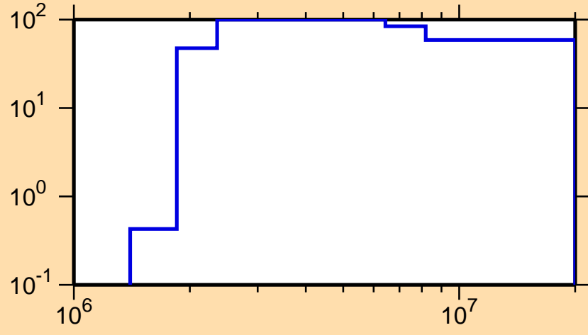
\Delta\sigma/\sigma vs. E for ^{256}\text{No}(n,p)
