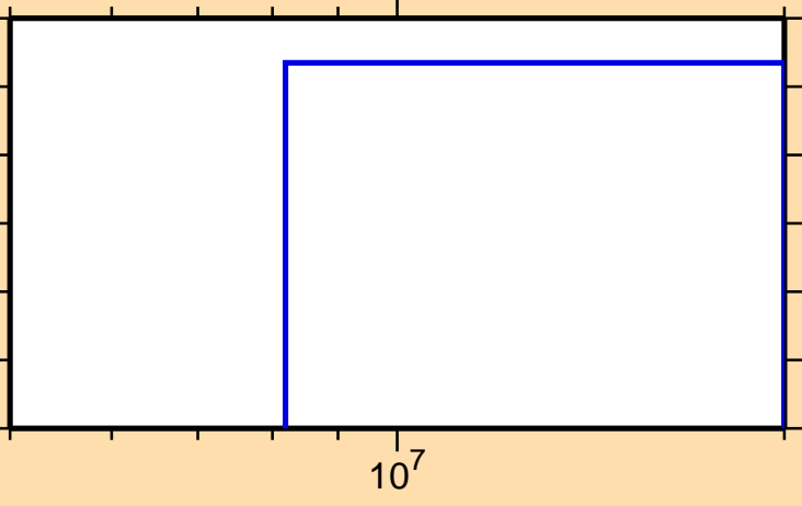
\sigma vs. E for ^{256}\text{No}(n,nt)
