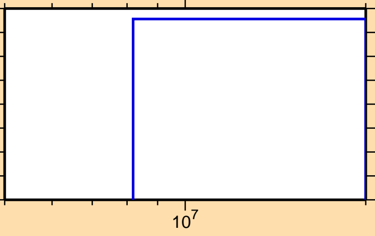
\sigma vs. E for ^{256}\text{No}(n,3n\alpha)
