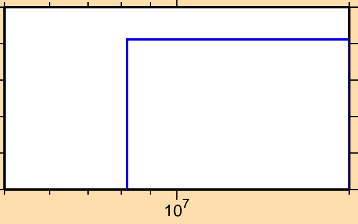
\sigma vs. E for ^{256}\text{No}(\text{mt } 34)
