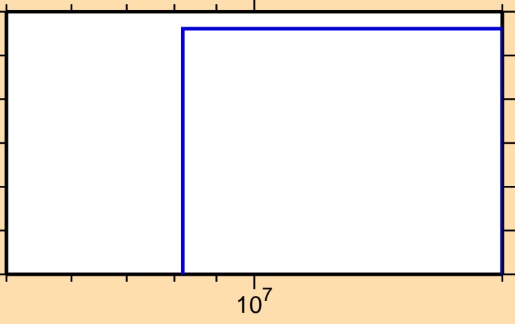
\sigma vs. E for ^{256}\text{No}(\text{mt117})
