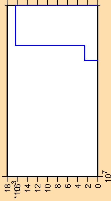
\Delta\sigma/\sigma vs. E for ^{257}\text{No}(\text{mt } 45)
