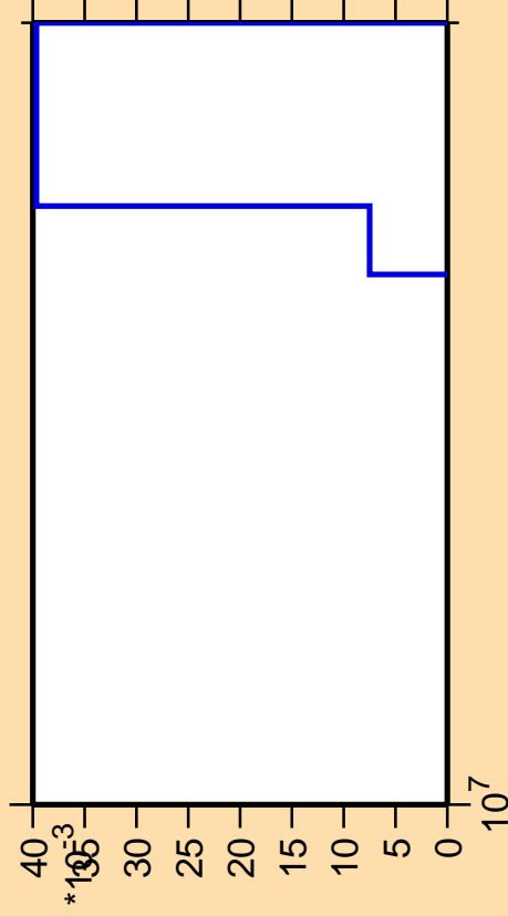
\Delta\sigma/\sigma vs. E for ^{257}\text{No}(\text{mt117})
