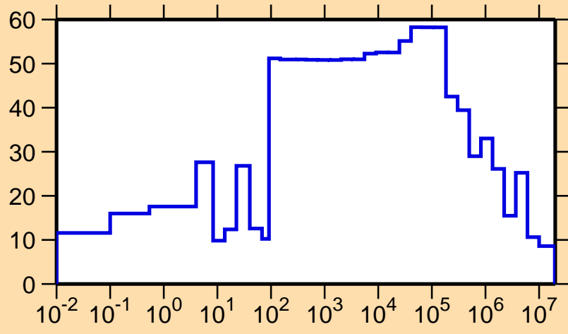
\Delta\sigma/\sigma vs. E for ^{257}\text{No}(n,el.)
