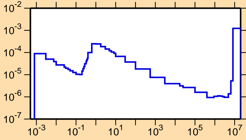
\sigma vs. E for ^{257}\text{No}(n,\alpha)
