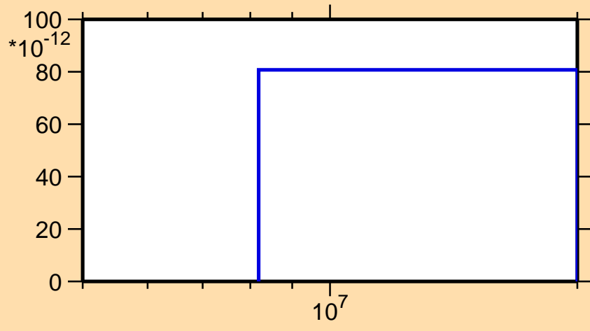
\sigma vs. E for ^{257}\text{No}(n,\text{He}3)
