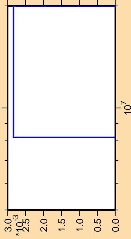
\Delta\sigma/\sigma vs. E for ^{257}\text{No}(\text{mt } 11)
