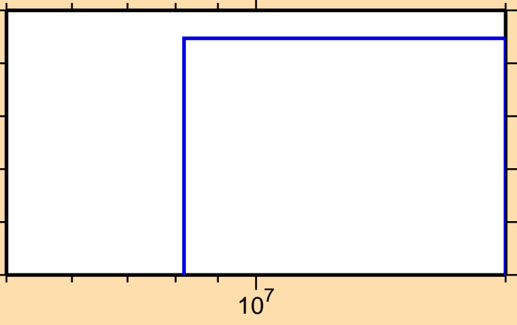
\sigma vs. E for ^{257}\text{No}(n,2np)
