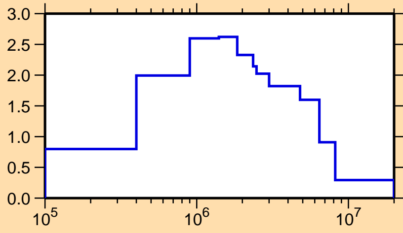
\sigma vs. E for ^{257}\text{No}(n,\text{inel.})
