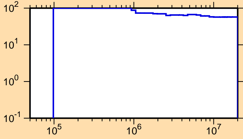
\Delta\sigma/\sigma vs. E for ^{259}\text{No}(n,\text{inel.})
