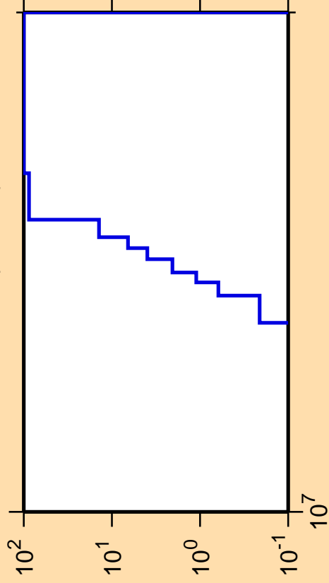
\Delta\sigma/\sigma vs. E for ^{259}\text{No}(n,\text{He}3)
