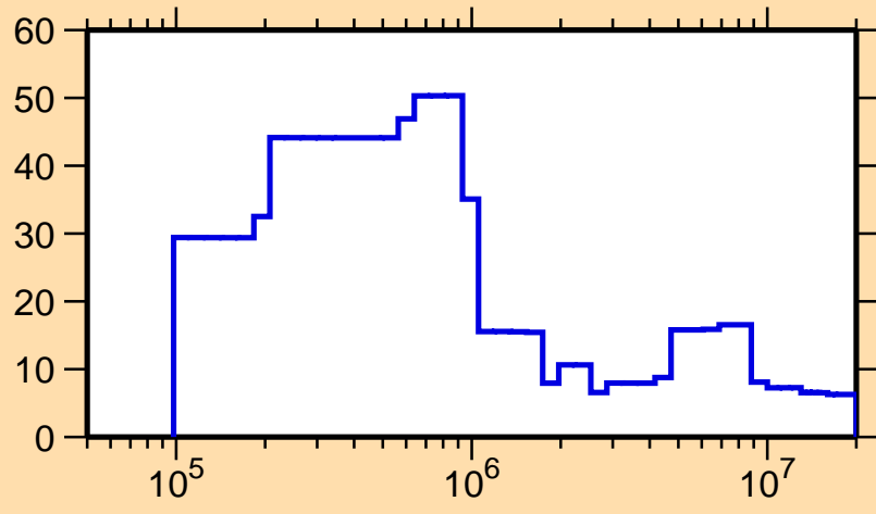
\Delta\sigma/\sigma vs. E for ^{259}\text{No}(n,\text{el.})
