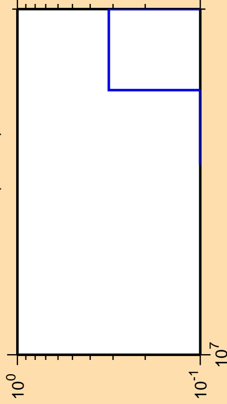
\Delta\sigma/\sigma vs. E for ^{259}\text{No}(\text{mt } 11)
