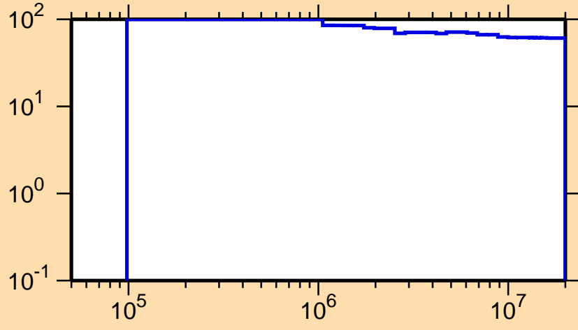
\Delta\sigma/\sigma vs. E for ^{259}\text{No}(n,n\text{cont.})
