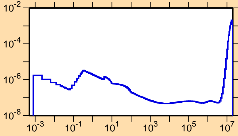
\sigma vs. E for ^{259}\text{No}(n,\alpha)
