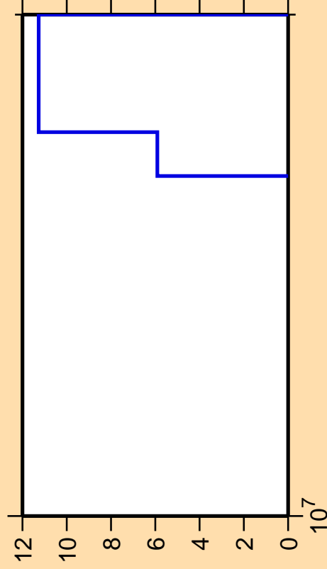
\Delta\sigma/\sigma vs. E for ^{259}\text{No}(n,p\alpha)
