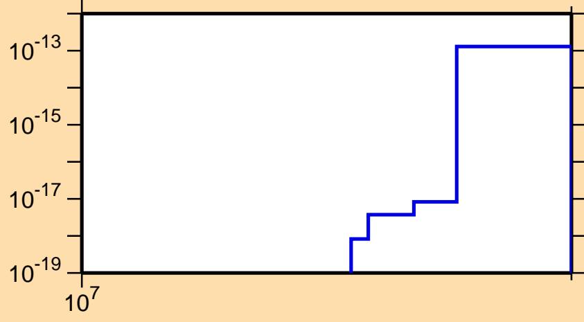
\sigma vs. E for ^{259}\text{No}(\text{mt } 11)
