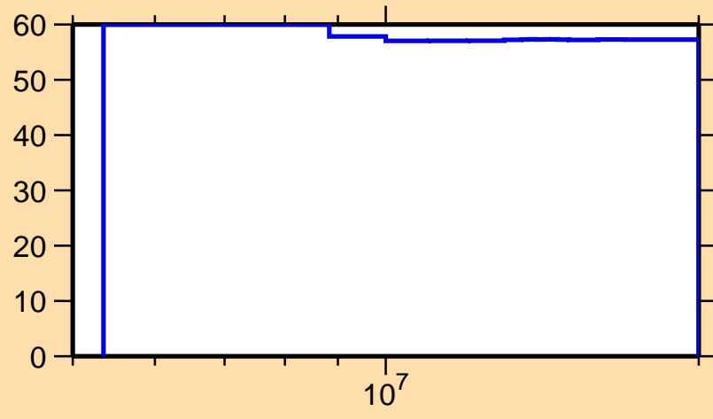
\Delta\sigma/\sigma vs. E for ^{259}\text{No}(n,\text{inel.})
