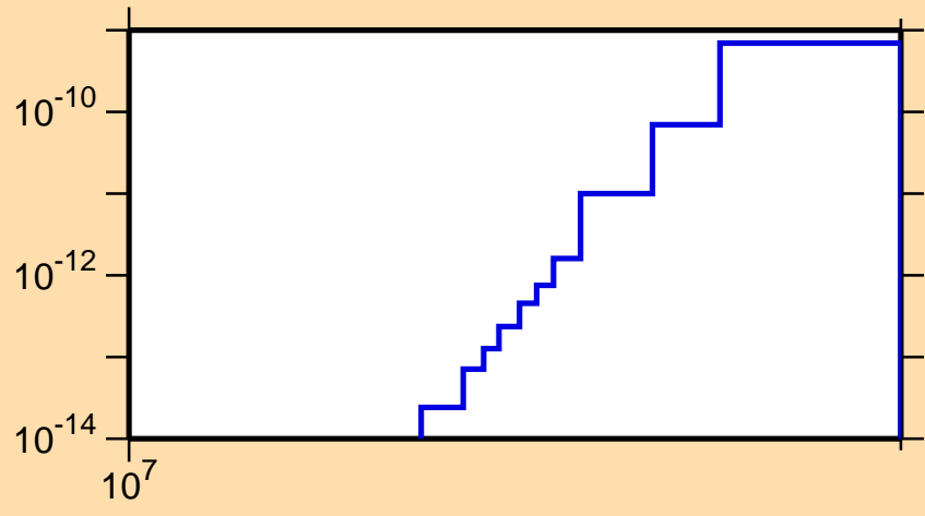
\sigma vs. E for ^{259}\text{No}(n,\text{He}3)
