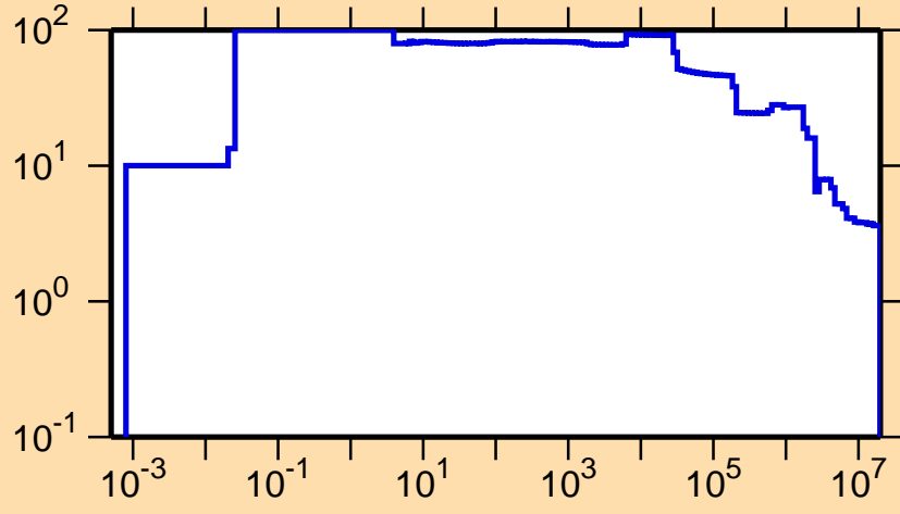
\Delta\sigma/\sigma vs. E for ^{259}\text{No}(n,\text{nonel.})
