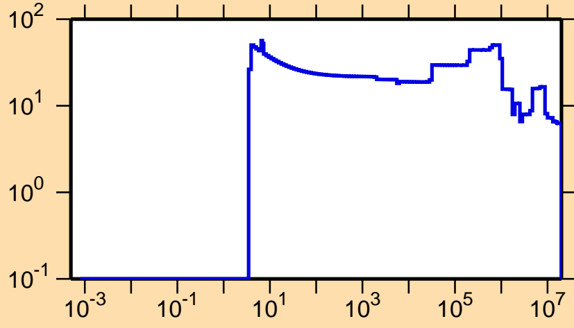
\Delta\sigma/\sigma vs. E for ^{259}\text{No}(n,\text{el.})
