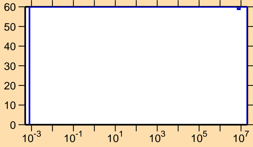
\Delta\sigma/\sigma vs. E for ^{259}\text{No}(n,\gamma)
