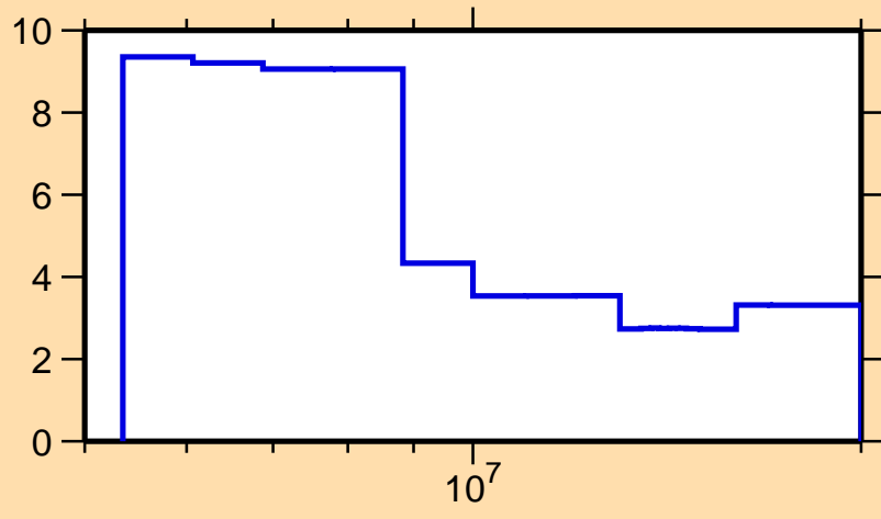
\Delta\sigma/\sigma vs. E for ^{259}\text{No}(n,\text{tot.})
