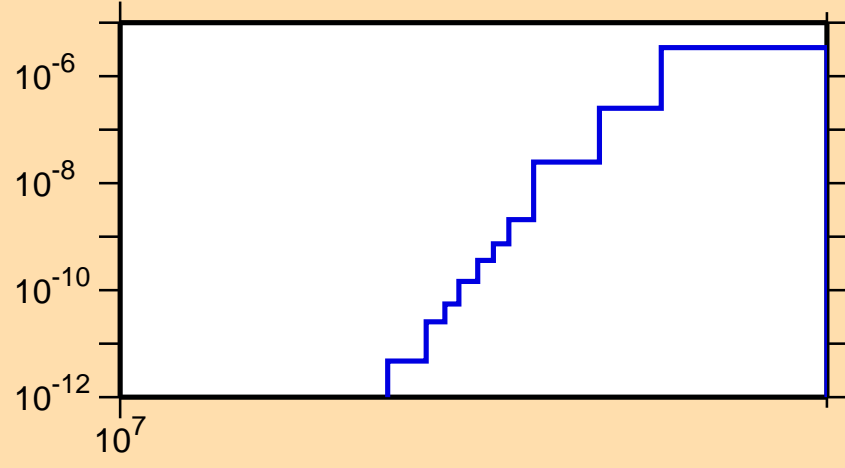
\sigma vs. E for ^{259}\text{No}(n,\text{nd})
