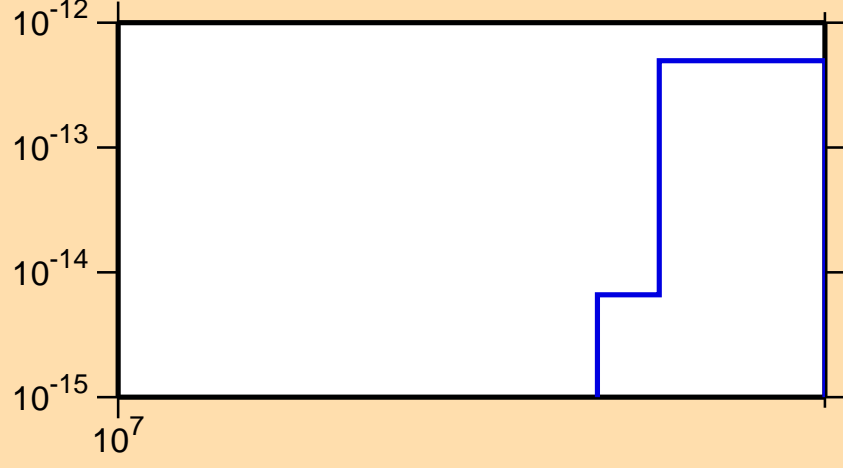
\sigma vs. E for ^{259}\text{No}(\text{mt } 34)
