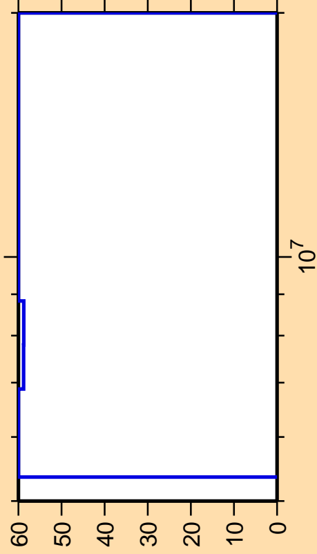
\Delta\sigma/\sigma vs. E for ^{259}\text{No}(n,\gamma)
