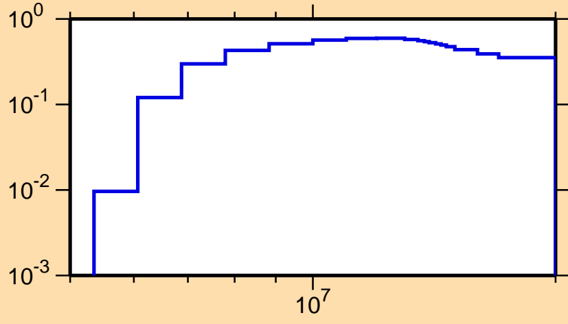
\sigma vs. E for ^{259}\text{No}(n,2n)
