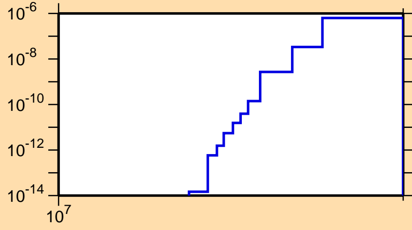
\sigma vs. E for ^{259}\text{No}(n,2np)
