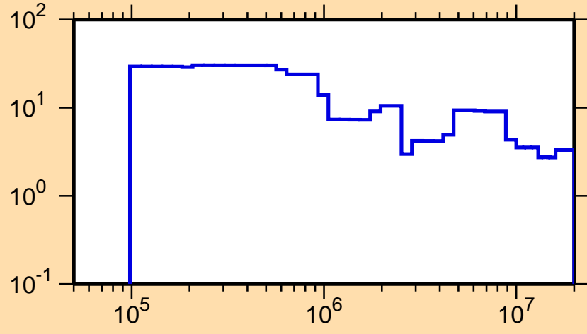
\Delta\sigma/\sigma vs. E for ^{259}\text{No}(n,\text{tot.})
