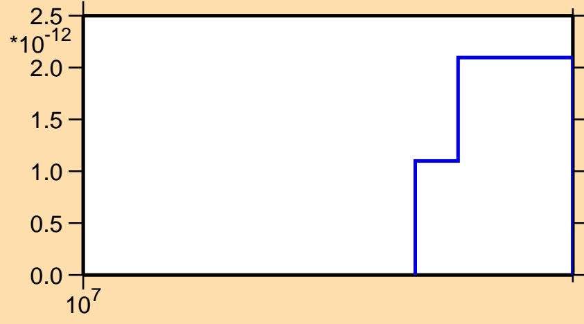
\sigma vs. E for ^{259}\text{No}(n,p\alpha)
