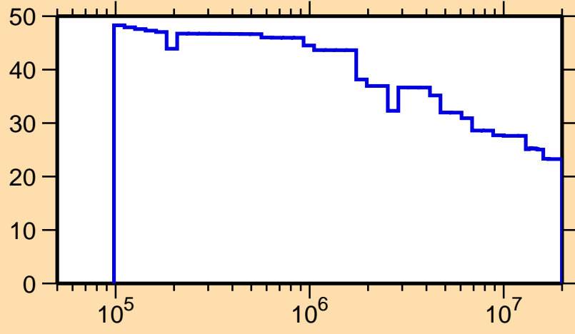
\Delta\sigma/\sigma vs. E for ^{259}\text{No}(n,f)
