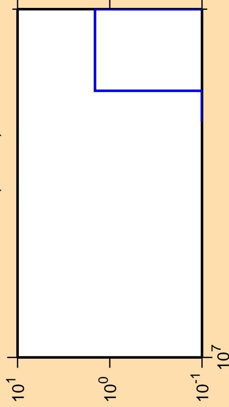
\Delta\sigma/\sigma vs. E for ^{259}\text{No}(\text{mt } 34)
