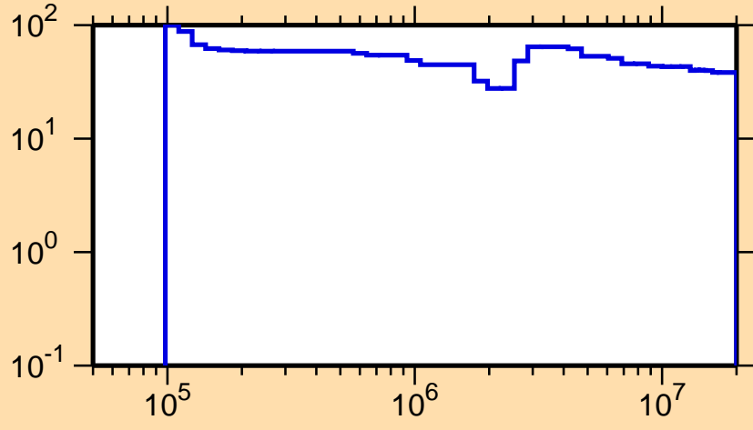
\Delta\sigma/\sigma vs. E for ^{259}\text{No}(n,n_1)
