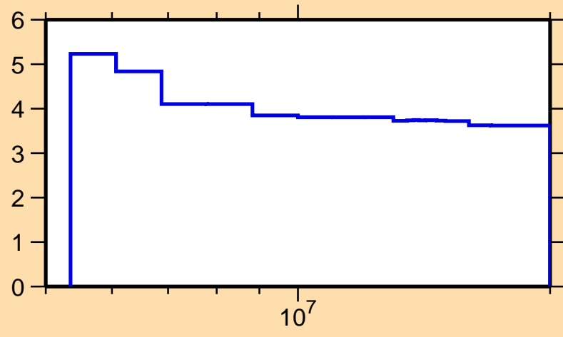
\Delta\sigma/\sigma vs. E for ^{259}\text{No}(n,\text{nonel.})
