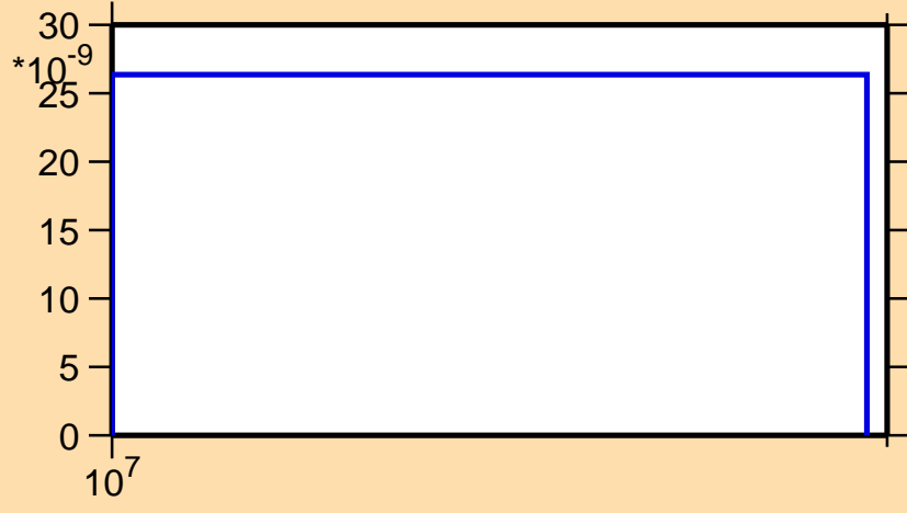
\sigma vs. E for ^{259}\text{No}(n,nt)
