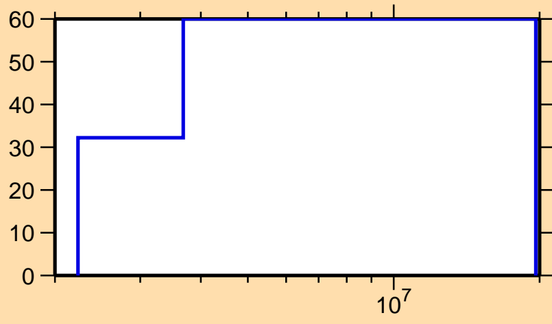
\Delta\sigma/\sigma vs. E for ^{259}\text{No}(n,p)
