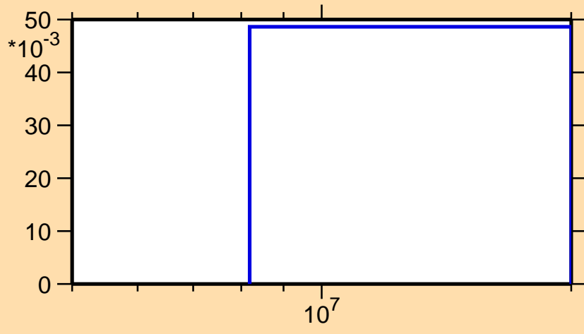
\sigma vs. E for ^{259}\text{No}(n,3n)
