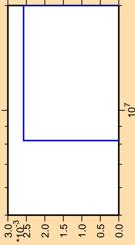
\Delta\sigma/\sigma vs. E for ^{259}\text{No}(\text{mt } 11)
