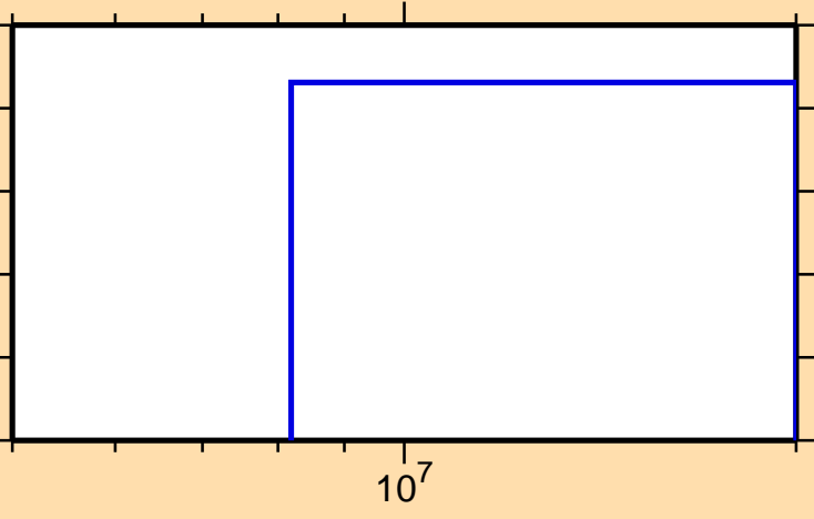
\sigma vs. E for ^{259}\text{No}(\text{mt } 34)
