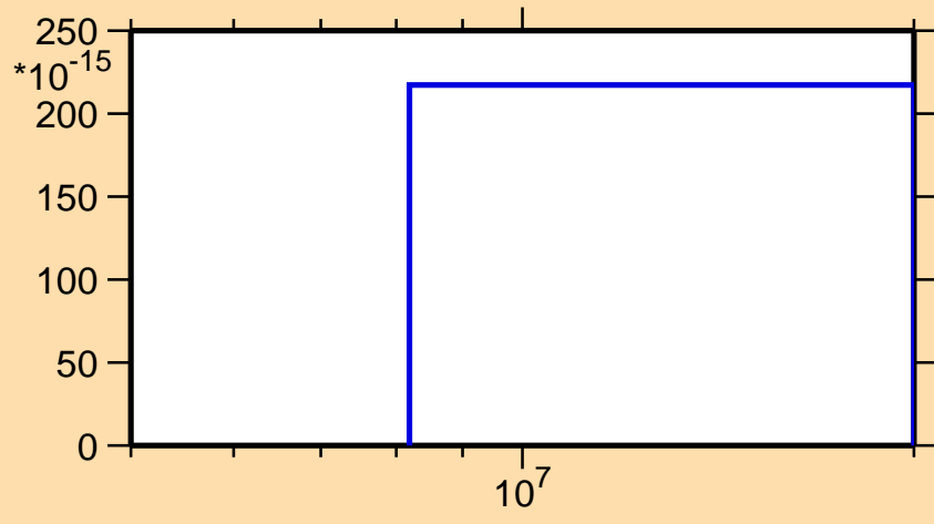
\sigma vs. E for ^{259}\text{No}(n,p\alpha)
