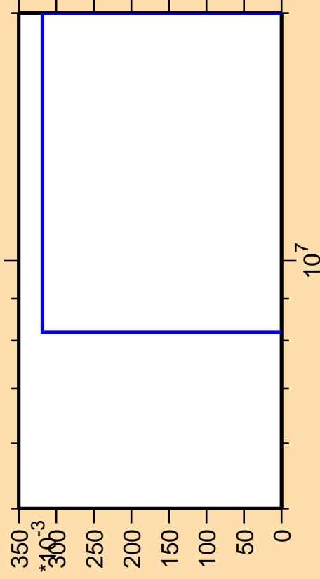
\Delta\sigma/\sigma vs. E for ^{259}\text{No}(n,p\alpha)
