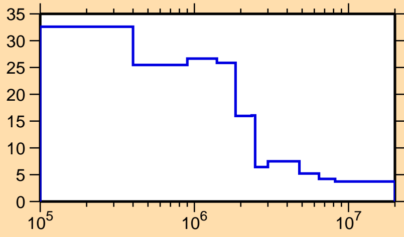
\Delta\sigma/\sigma vs. E for ^{259}\text{No}(n,\text{nonel.})
