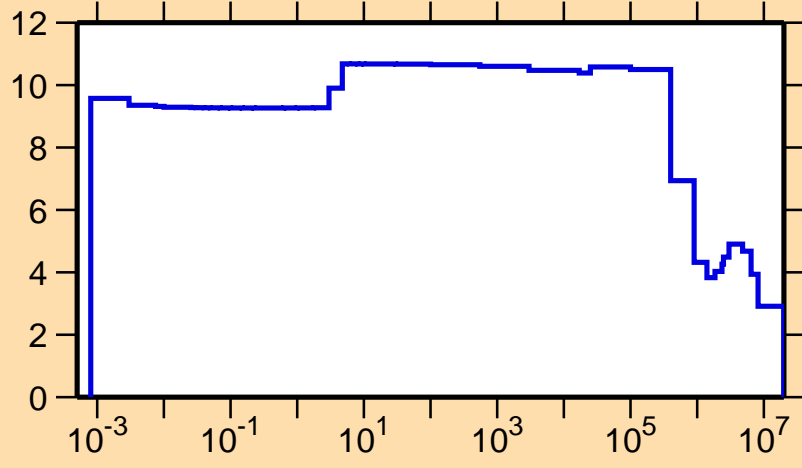
\sigma vs. E for ^{259}\text{No}(n,\text{el.})
