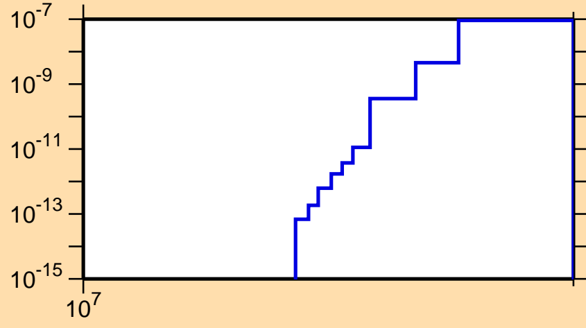
\sigma vs. E for ^{261}\text{No}(n,2np)
