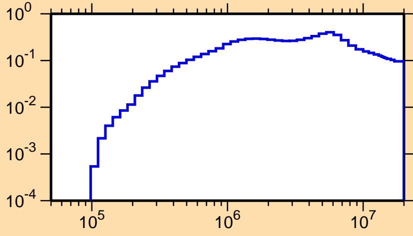
\sigma vs. E for ^{261}\text{No}(n,n\text{cont.})
