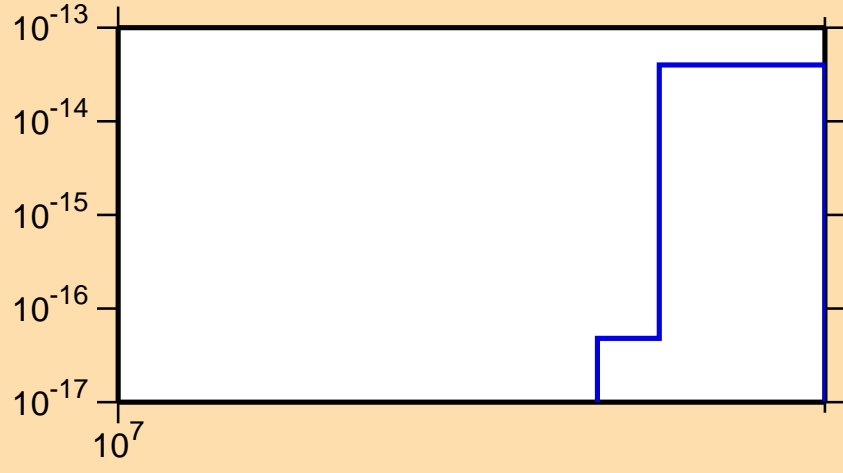
\sigma vs. E for ^{261}\text{No}(\text{mt } 11)
