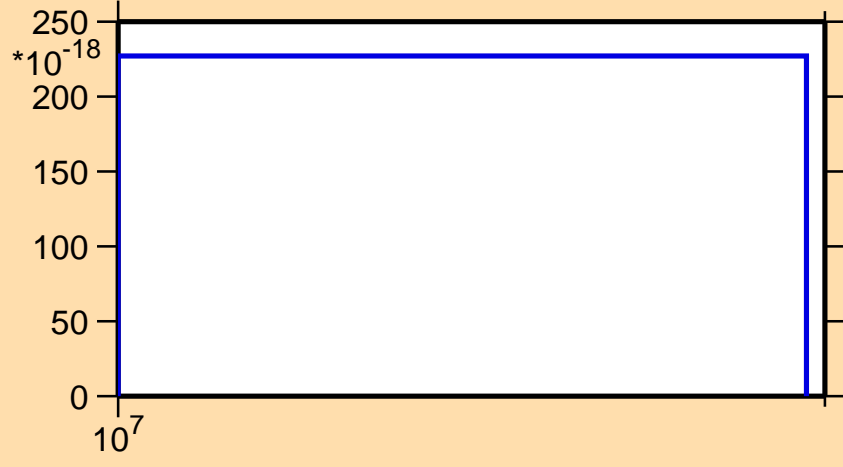
\sigma vs. E for ^{261}\text{No}(\text{mt } 11)
