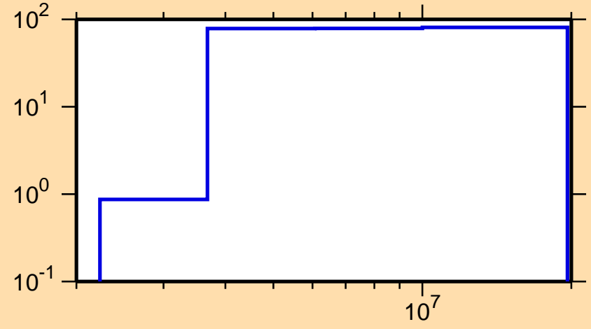
\Delta\sigma/\sigma vs. E for ^{261}\text{No}(n,p)
