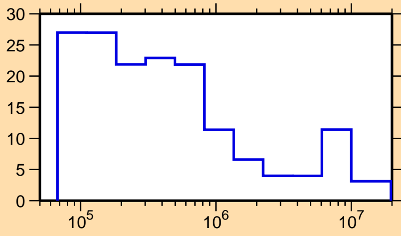
\Delta\sigma/\sigma vs. E for ^{261}\text{No}(n,\text{tot.})
