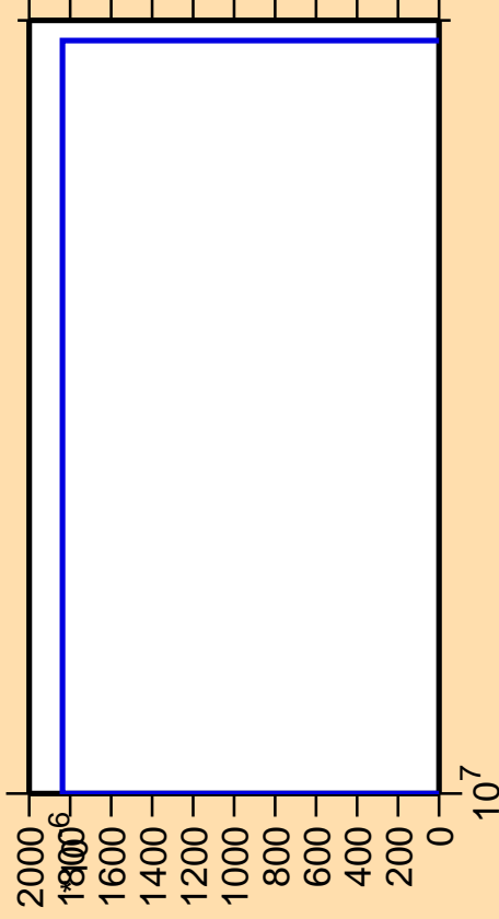
\Delta\sigma/\sigma vs. E for ^{261}\text{No}(\text{mt } 11)
